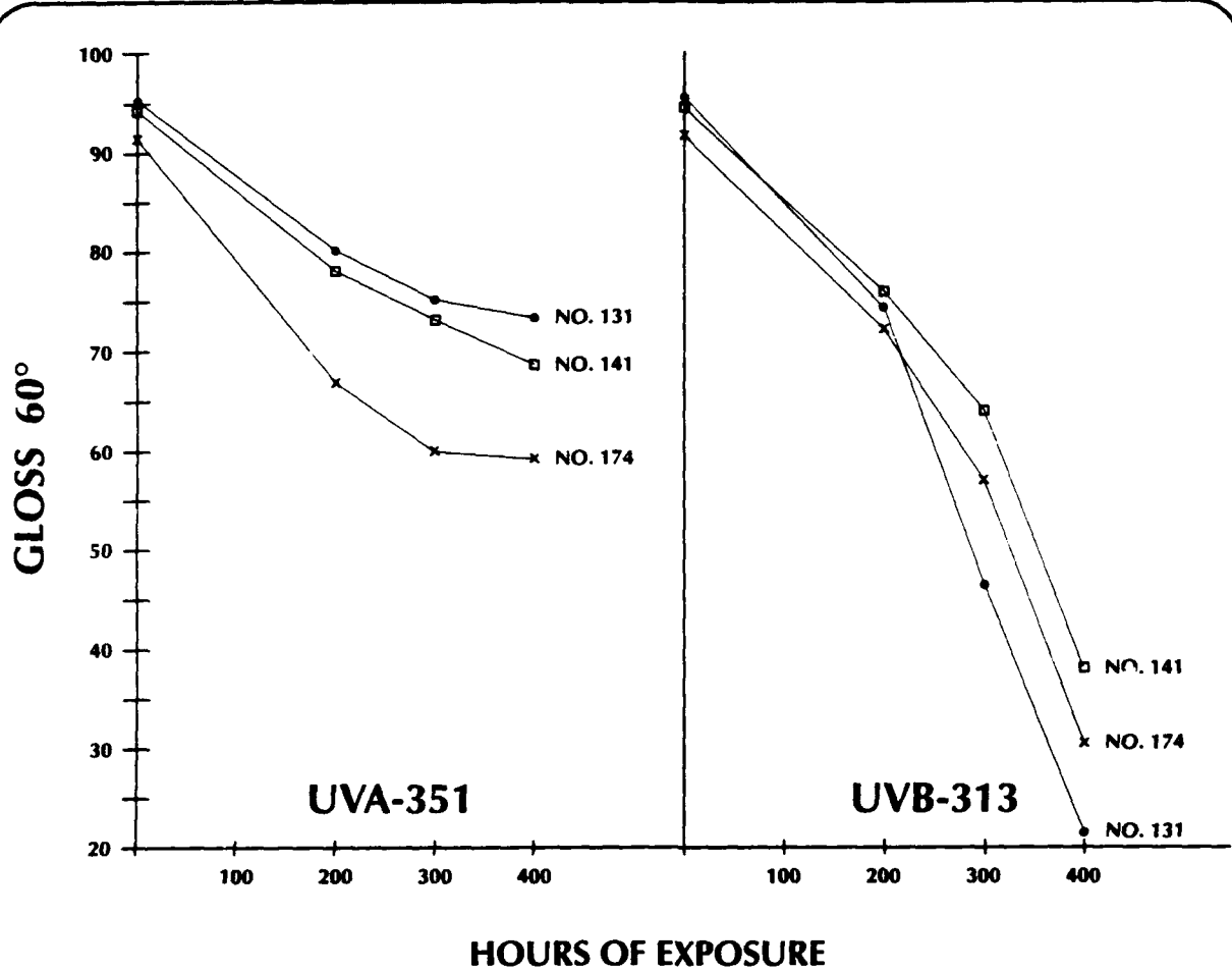
Figure 3. Gloss Change for Three Orange Formulations
