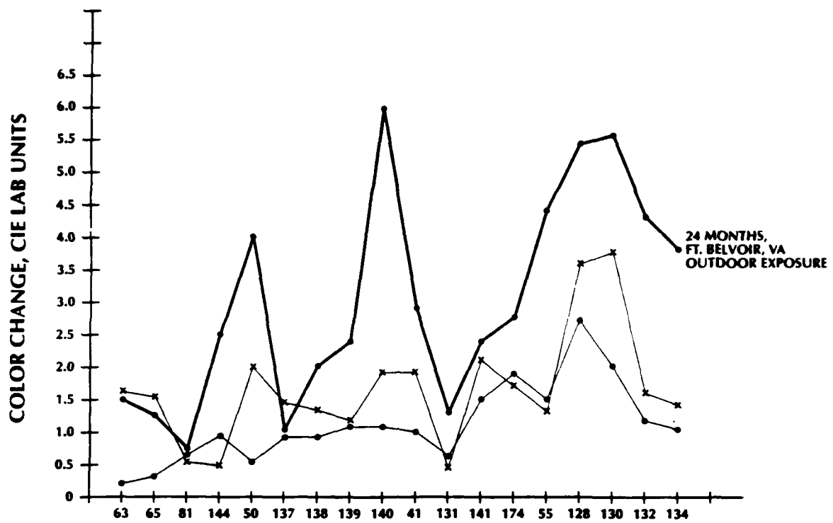
Laboratory Formulas After 24 Months Outdoor Exposure at Fort Belvoir, VA.
