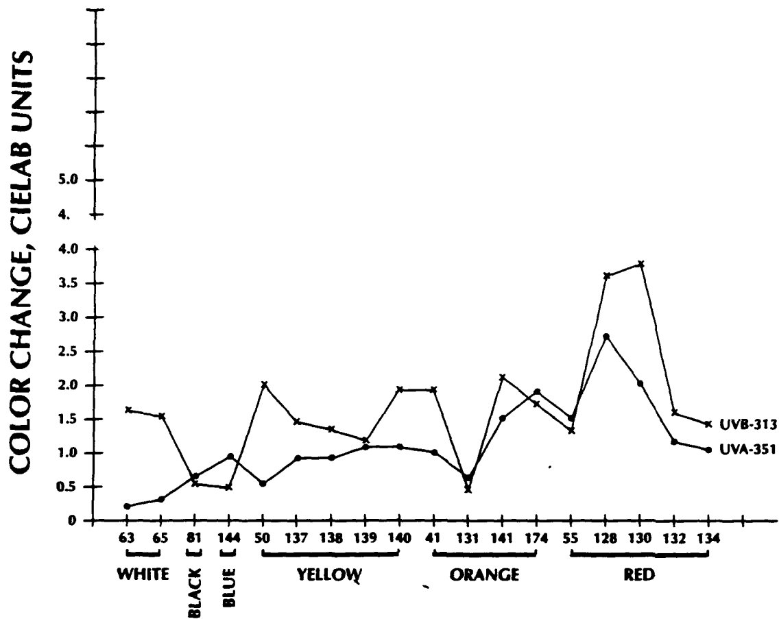
Figure 5. Color Change After Exposure
