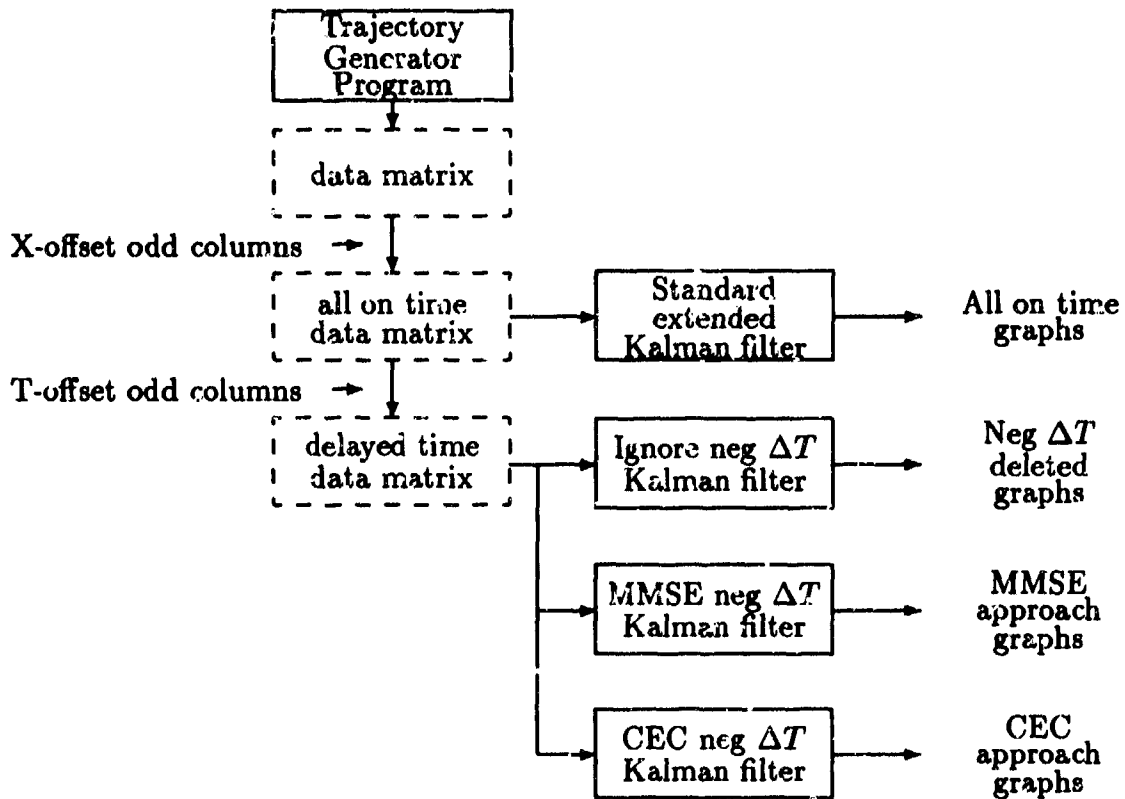
Figure 5-2. Basic Outline of Simulation
