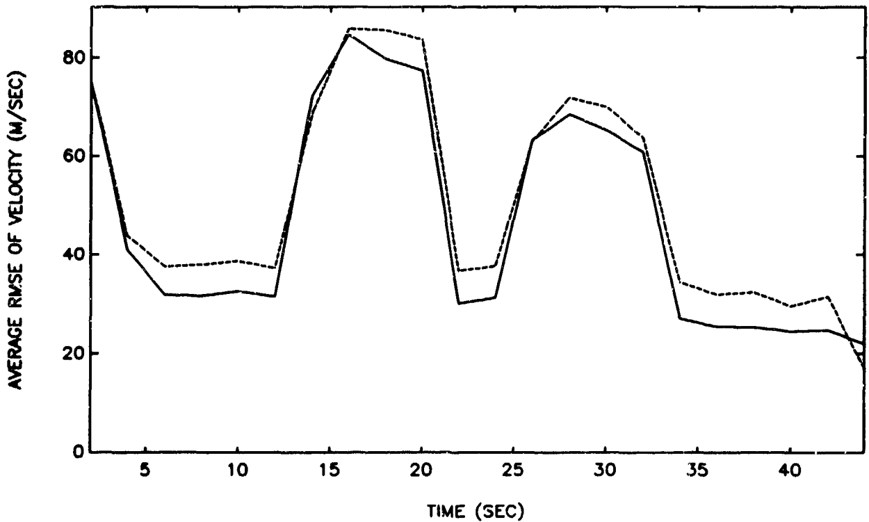
Figure 5-5. Tracking Results for Cases 3 and 4
