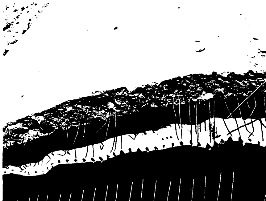
Figure 157. View of transverse failure plane in arch, PAS-2.
