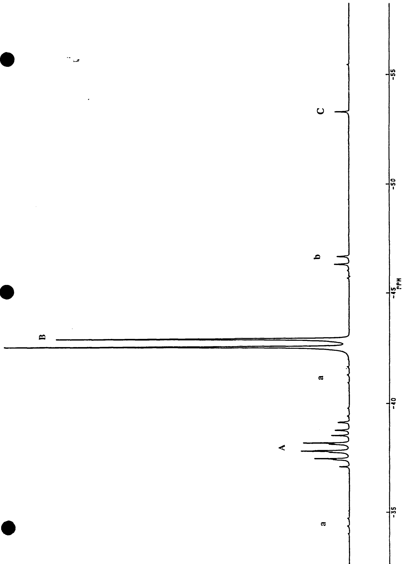
Figure 5. ^{19}\text{F} NMR of \text{F}_5\text{TeNH}_2 in \text{BrF}_3 at -50^\circ\text{C} ; (A), (B), \text{AB}_4 pattern due to F-on-Te(VI), (a),
