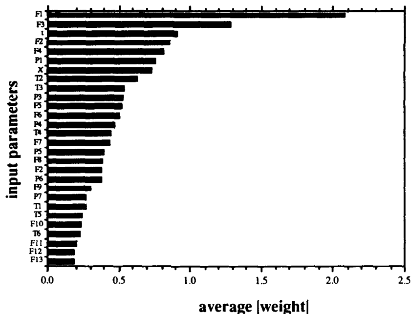
Figure 3. Average weights from linear networks (NN1): correlation of inputs to layer thickness.
