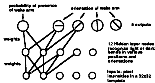
Figure 3. Feature detection neural network (nn1).
