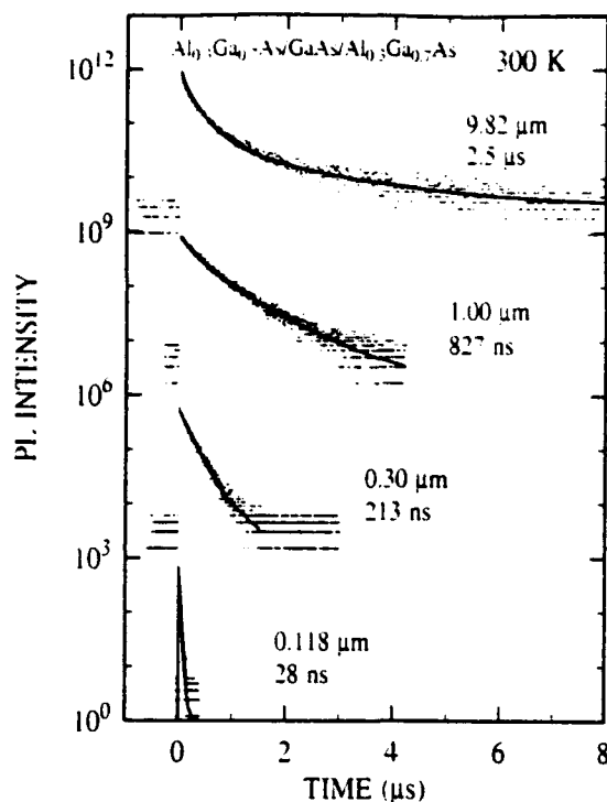
FIG. 4. Decay kinetics for GaAs/Al 0.3 Ga 0.7 As double heterostructures with 9.82 μm, 1.00 μm, 0.30 μm, and 0.118 μm GaAs layer thicknesses at room temperature. Lifetimes shown represent the 1/e constant for the exponential tails of the decays, and were obtained through least-squares fits of the data to Eq. (3).
