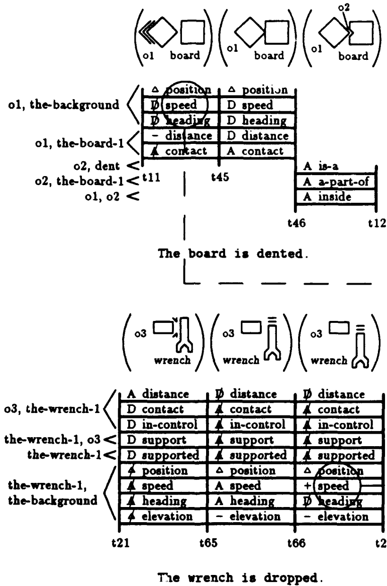
Figure 4: Event traces for the description: "The board is dented. The wrench is dropped." A partial match between the two traces is indicated.
