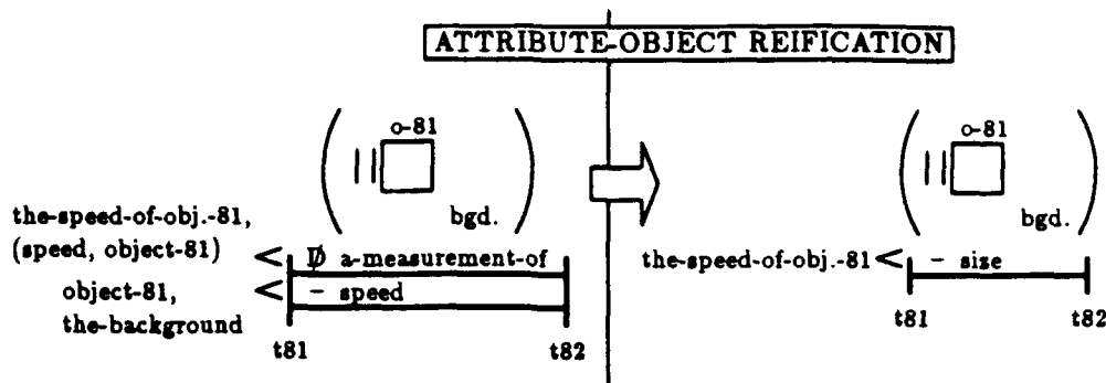
Figure 10: An attribute-object reification transformation.
