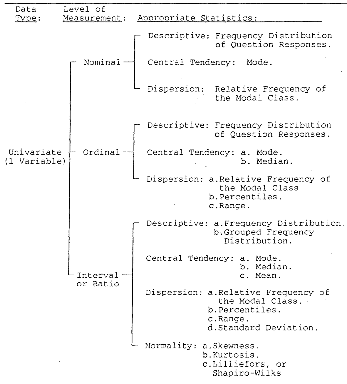
FIGURE 1. Univariate Statistics for Survey Data
