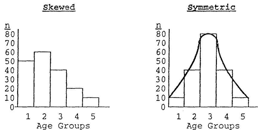
FIGURE 2. Skewed vs. Symmetric Bell-Shaped Distributions
