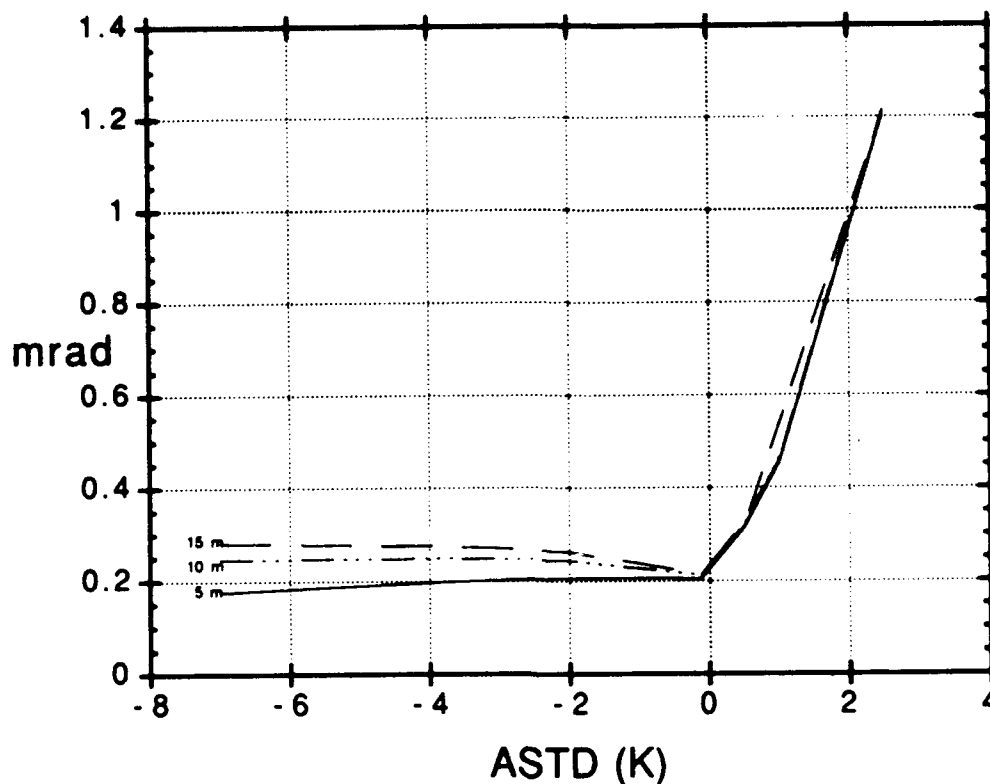
Fig. 43 — Apparent direction of the target when it is at the MIVR (for negative ASTD) or at the inductive range shown for positive ASTD in Fig. 41
