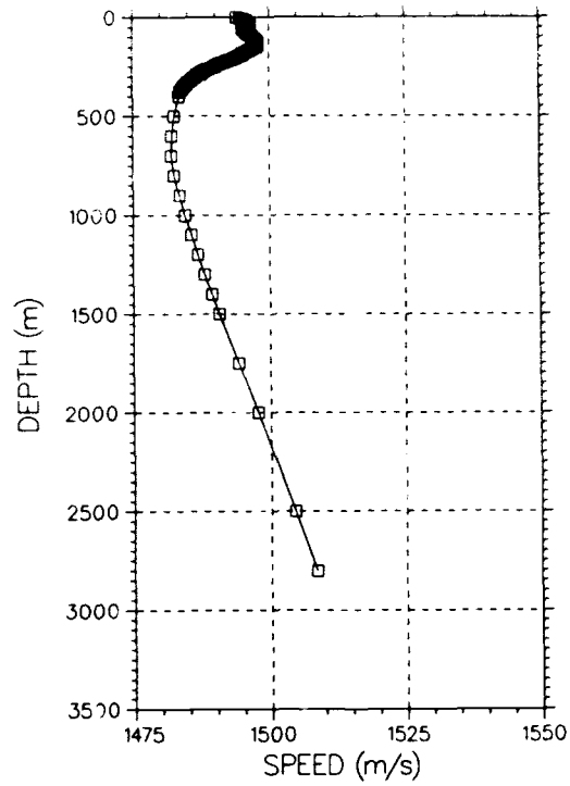
Fig. A2—Flight 2, Site A's composite sound speed profile (in-situ extended via the GDEM database)
