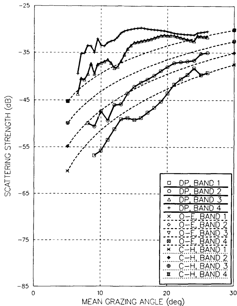
Fig. 14—Flight 2, Site B, 18.0 m/s mean wind speed measured surface scattering strengths (solid lines) compared to both the Ogdén-Erskine empirical algorithm (dashed lines) and the Chapman-Harris empirical formula (dotted lines)
