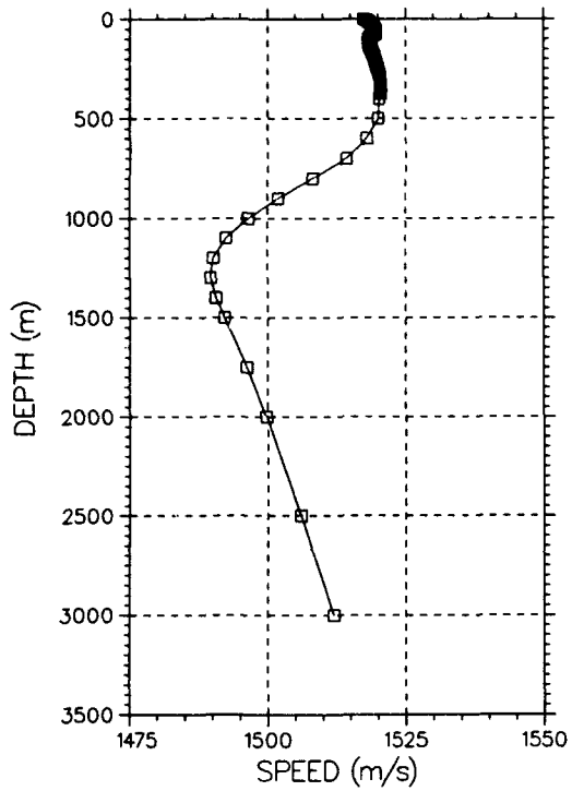
Fig. A9—Flight 6, Site E's composite sound speed profile (in-situ extended via the GDEM database)
