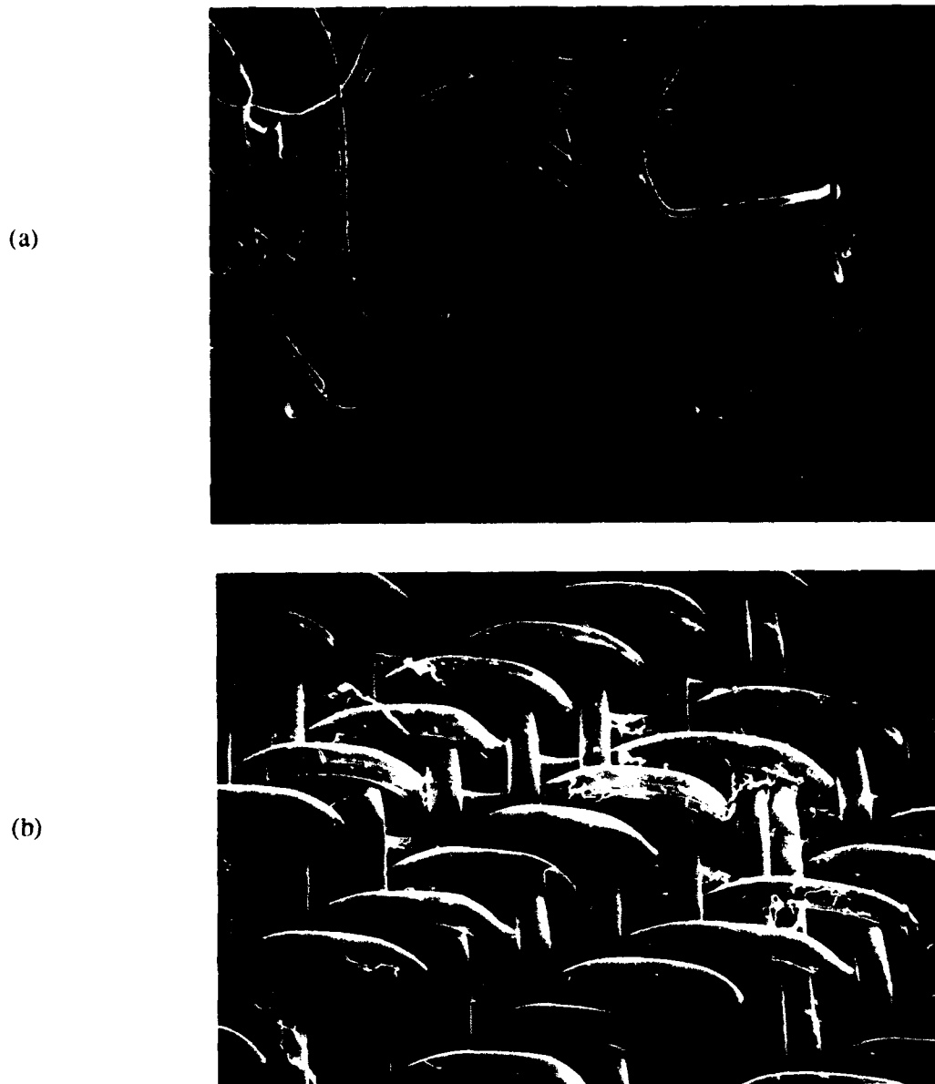
Figure 9. Photomicrographs showing (a) woven and (b) nonwoven geotextile fibers.
