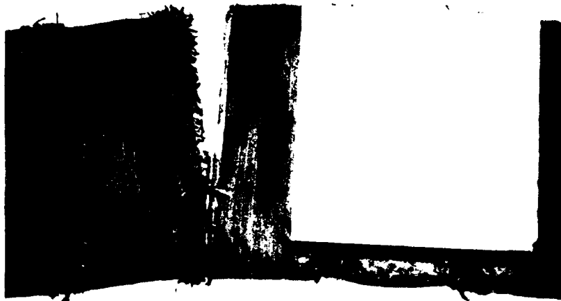
Figure 37. Failure of peel test specimen by fabric tearing outside of bond area.
