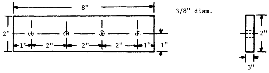
RIBBED PLATE
