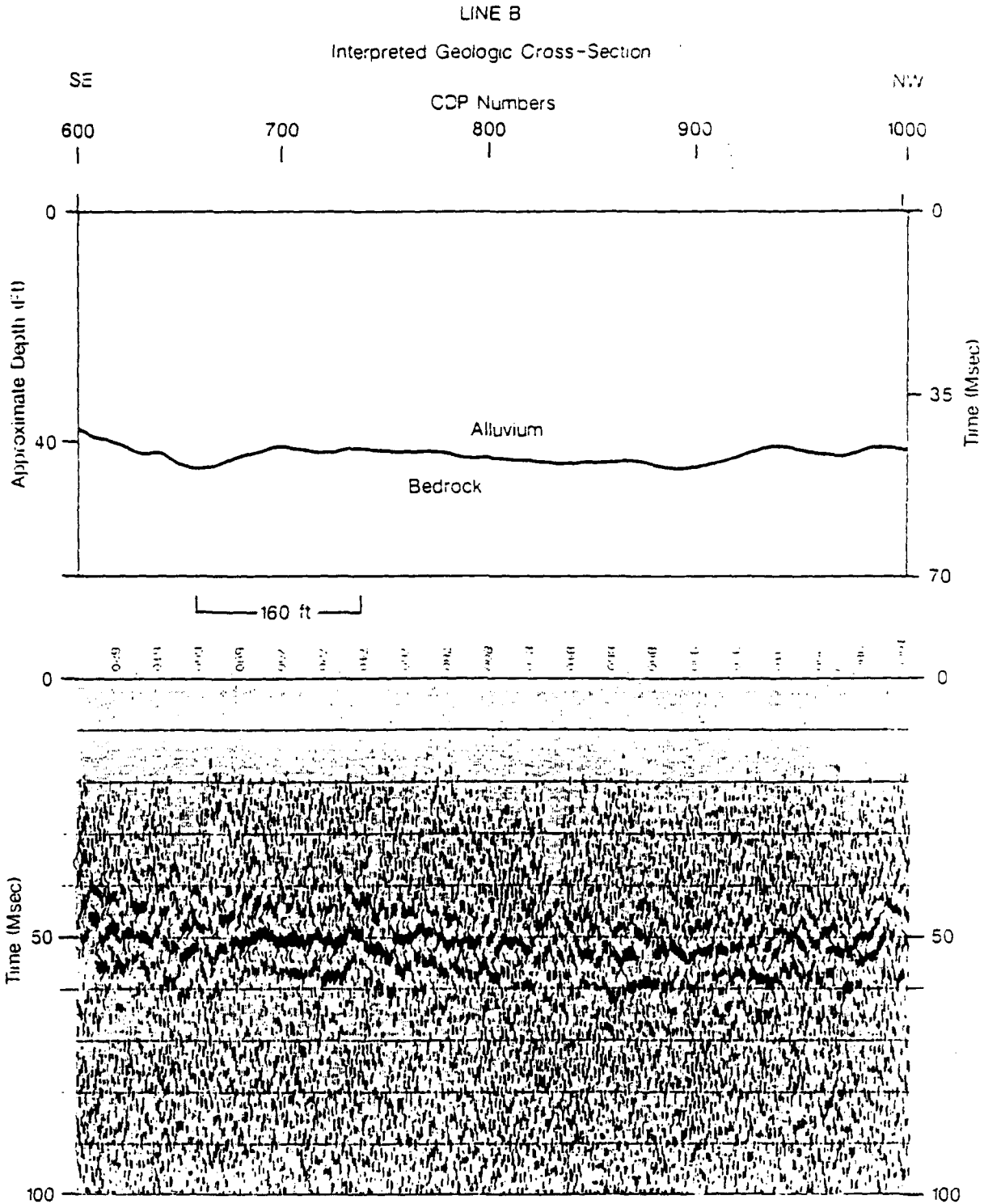
Figure 3. Seismic section and geologic cross-section of Line B. Each CDP trace is separated by 2 feet and possesses at least 6 fold and as much as 12 fold redundancy. The poor coherency in the bedrock reflection wavelet from trace to trace could be a result of the multiple roads and trails crossed during the acquisition of Line B.
