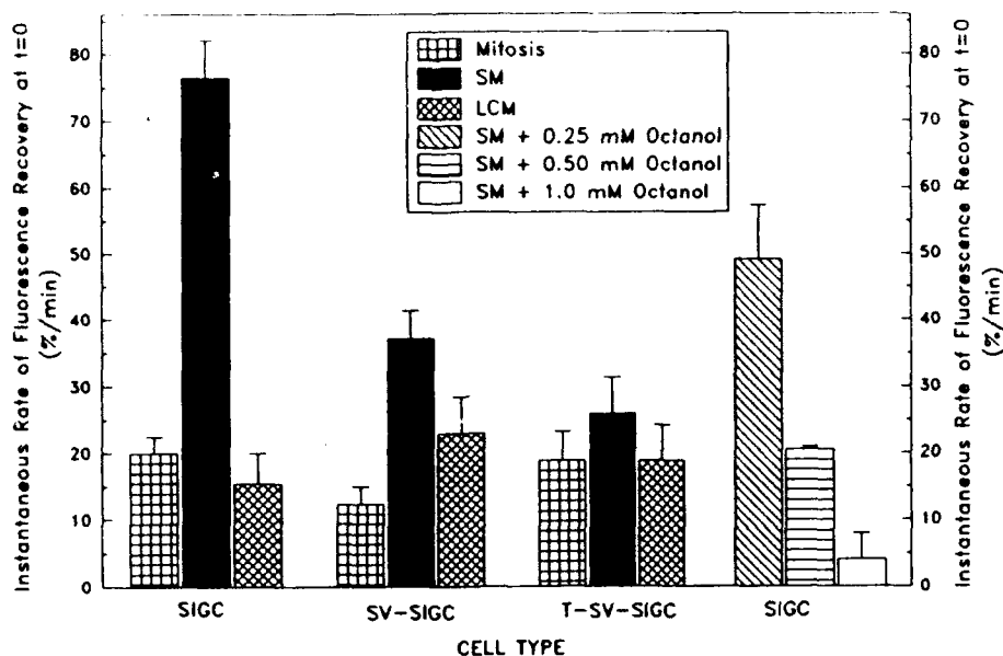
FIG. 8. Comparison between all cell systems of the estimated instantaneous rates of recovery at the time of the first postbleach scan, I'(0)/I(0) , from (1, 4) sampling. Unless otherwise noted, all cells were cultured in SM and scanned during interphase. The notation SM refers to cell systems in standard conditions, i.e., SM in interphase. LCM, mitosis, and octanol systems were scanned 12 h after switching from SM to LCM, during the metaphase plate stage and immediately after the addition of octanol, respectively. Error bars represent the standard deviation (SD) of the estimate, I'(0)/I(0) . The vertical axis is 100 \times I'(0)/I(0) where I(0) is the intensity of fluorescence at the t = 0 and I' is the derivative of I .
