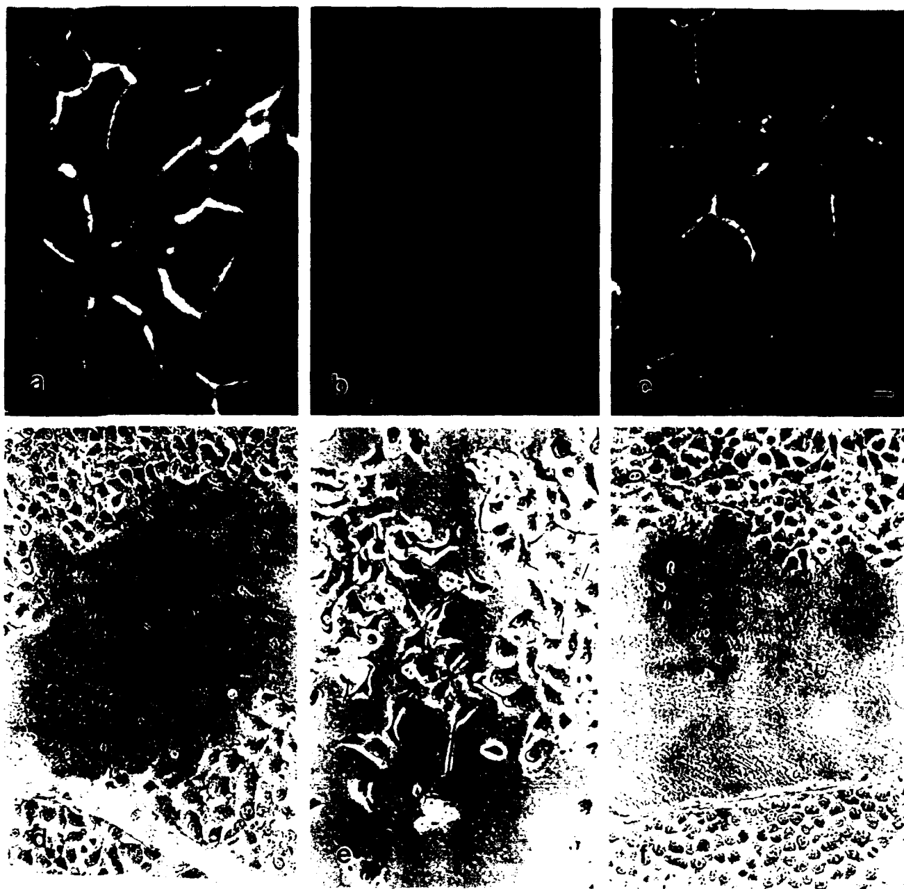
Fig. 1. A reversible loss of desmosomes in SIGC using antibody to desmoglein. (a-c) Fluorescence microscopy of SIGC cells cultured in SM for 48 h (a), switched to LCM for 4 h (b), and switched back to SM for 4 h (c). (d-f) Phase-contrast microscopy of SIGC monolayers. (d) Wounding as cells move into cell-free areas (wound) in the culture dishes. Cells were cultured in SM for 48 h, and media was replaced with fresh SM (d) or LCM (e) immediately prior to scraping monolayers with a pipet tip to produce a wound. In SM (d), cells were linked together and moved as an epithelial sheet. In LCM (e), cells detached from the wound nonlayer. (f) A characteristic SIGC epithelial pattern of movement was seen after return to SM, i.e., SM cells swam to the wound nonlayer, and allowed 10 h recovery → wound → photograph. Bars: (a-c) 5 \mu m; (d-f) 20 \mu m.
