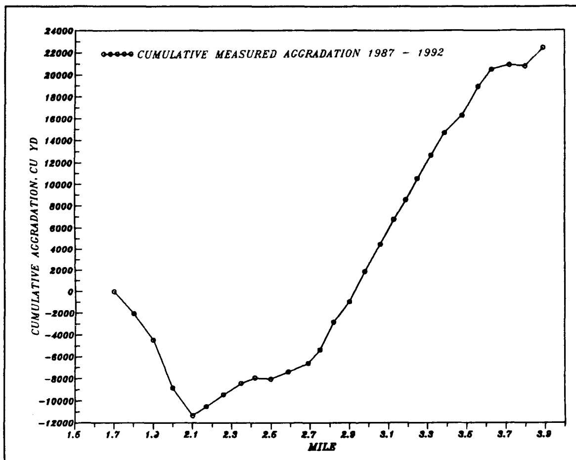
Figure 5. Measured accumulated aggradation in bypass channel between 1987 and 1992
