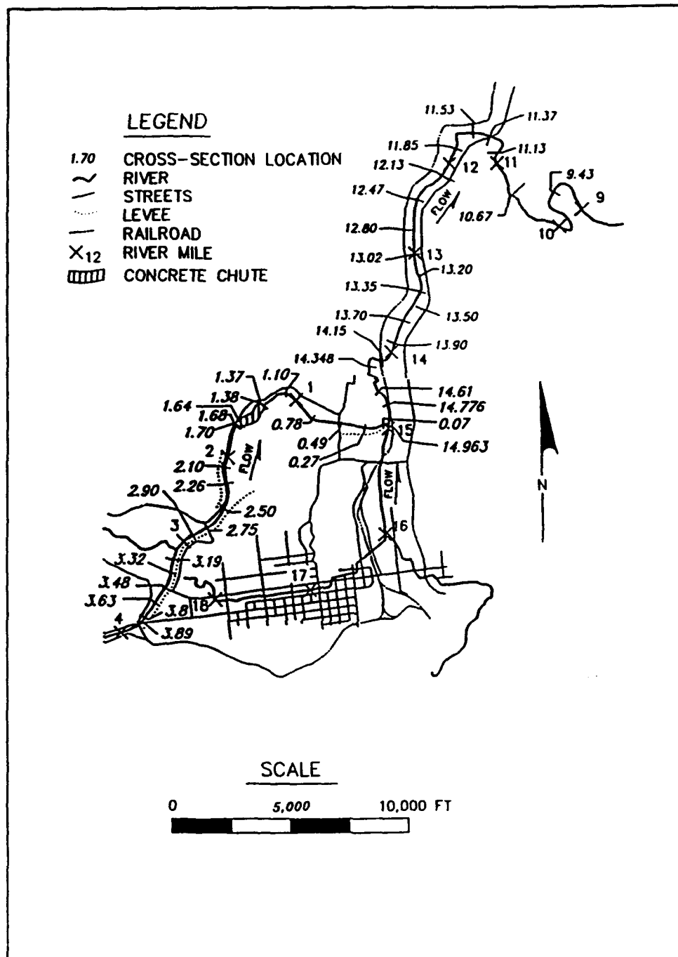
Figure 3. Cross-section locations
