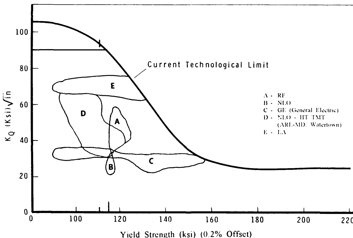
Figure 13. RAD for U-0.75 wt% Ti K_Q versus YS (0.2%)
