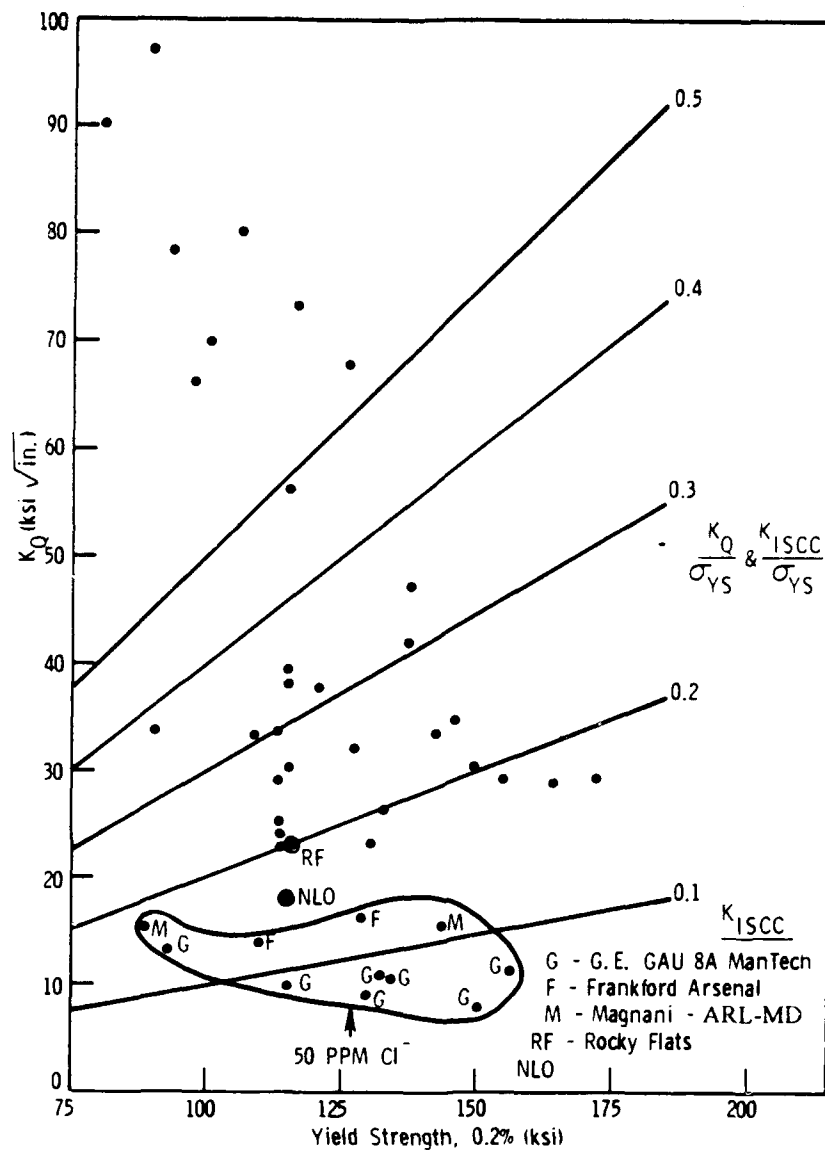
Figure 14. SCC and K_Q RAD for U-0.75 wt% Ti alloys
