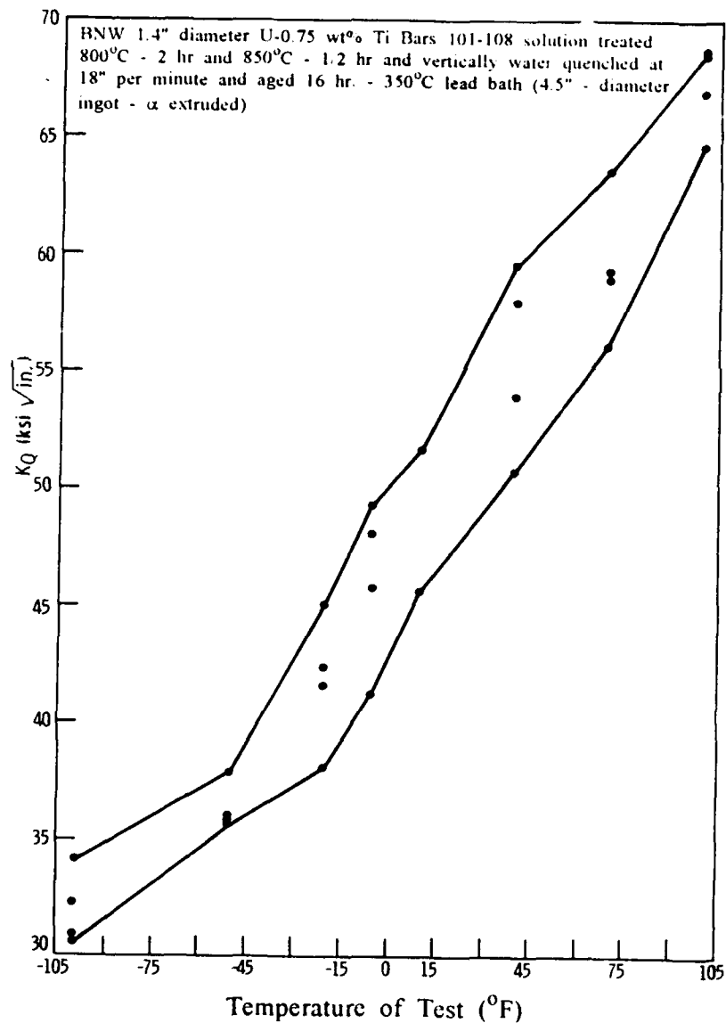
Figure 12. Fracture toughness of aged U-0.75 wt% Ti BNW bars versus temperature of test
