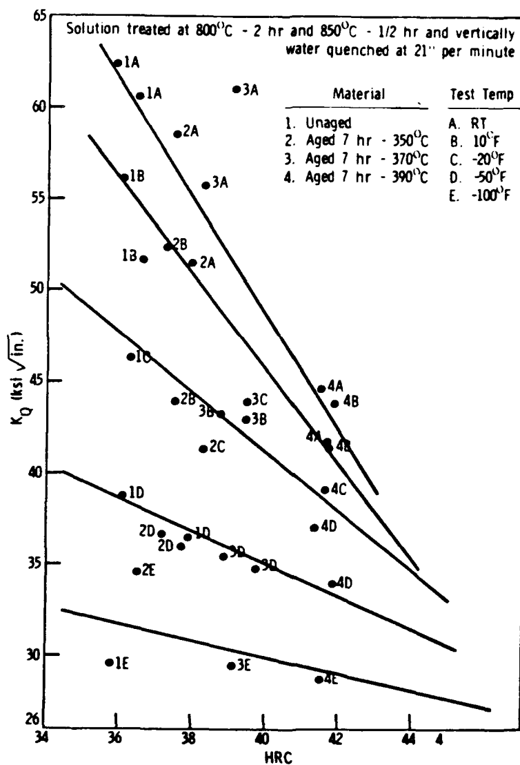
Figure 9. Fracture toughness of aged U-075 wt% Ti N 2 O bars (Charpy - K_Q ) versus HRC.
