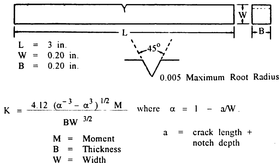
Figure 1. Specimen geometry and equation for K values
