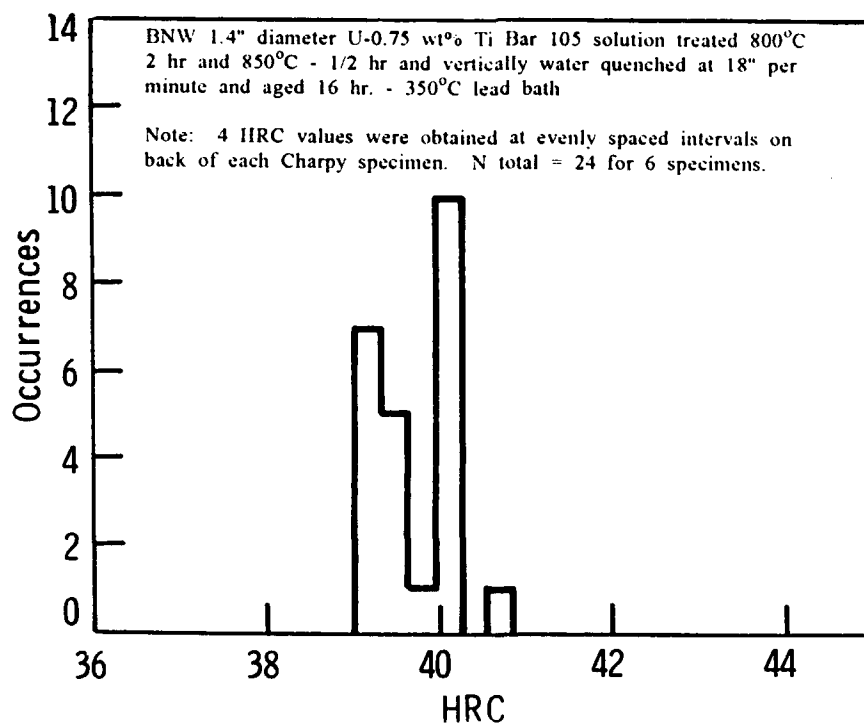
Figure 10. Frequency of Rockwell C readings versus HRC.
