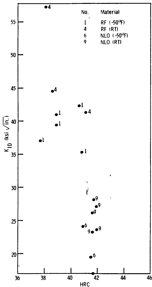
Figure 7. Dynamic fracture toughness of aged U-0.75 wt% Ti RF and NLO penetrators versus HRC
