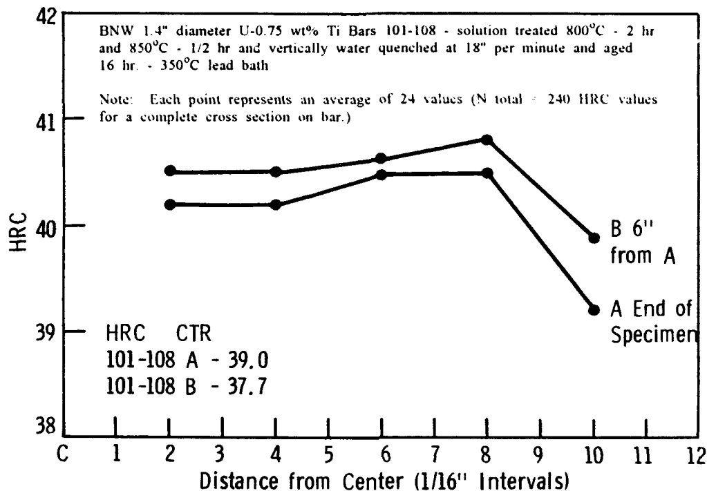
Figure 11. Transverse Rockwell C Hardness versus distance from center.
