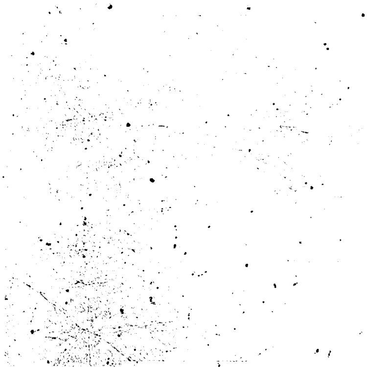
Figure 3. U-0.75 wt% Ti (RF) lower nose section - solution treated at 800°C for two hours, 850°C for one-half hour, vertically water quenched 18 inches per minute, aged (lead bath) for 16 hours at 350°C Mag 100X
