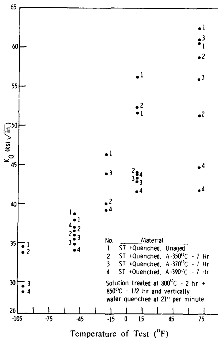
Figure 8. Fracture toughness of aged U-0.75 wt% Ti NLO bars versus temperature of test.
