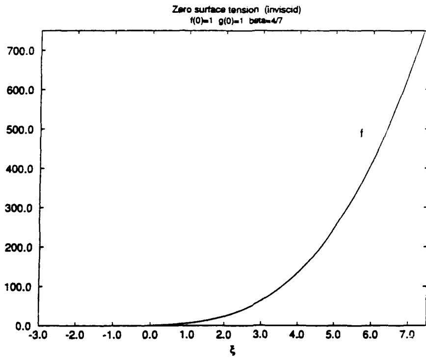
• Figure 1 Inviscid jet with zero surface tension; similarity solution f(\xi) .
