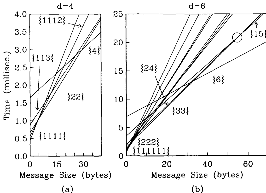
Figure 1: Run times for d = 4, 6 . In this particular example, \lambda = 100 , \delta = 10 ( \mu\text{sec.} ) and \tau = 2 , \rho = 1 ( \mu\text{sec./byte} ). Circle indicates the point of intersection of all partitions of cardinality 2: \{33\} , \{24\} and \{15\}
