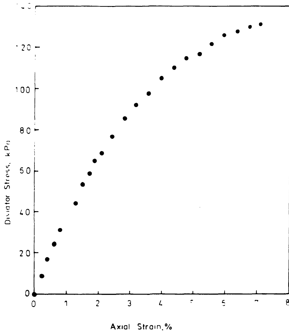
Fig. 6.1 Deviator stress vs. Axial strain (oc).
