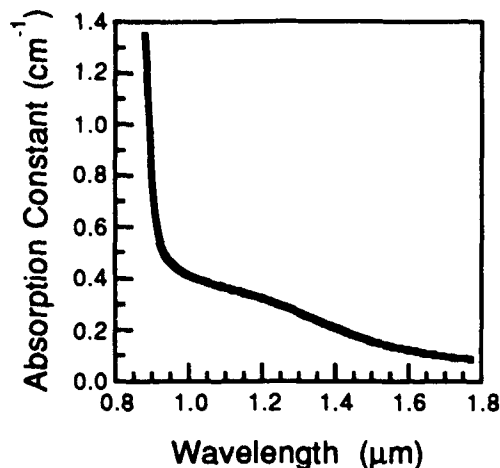
Fig. 1 Absorption spectrum of CdTe:In.
