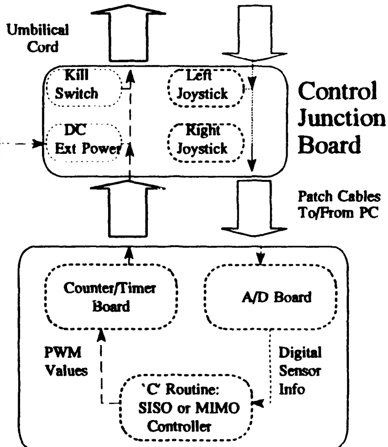
Figure 4 Archytas UAV Ground Equipment Block Diagram
