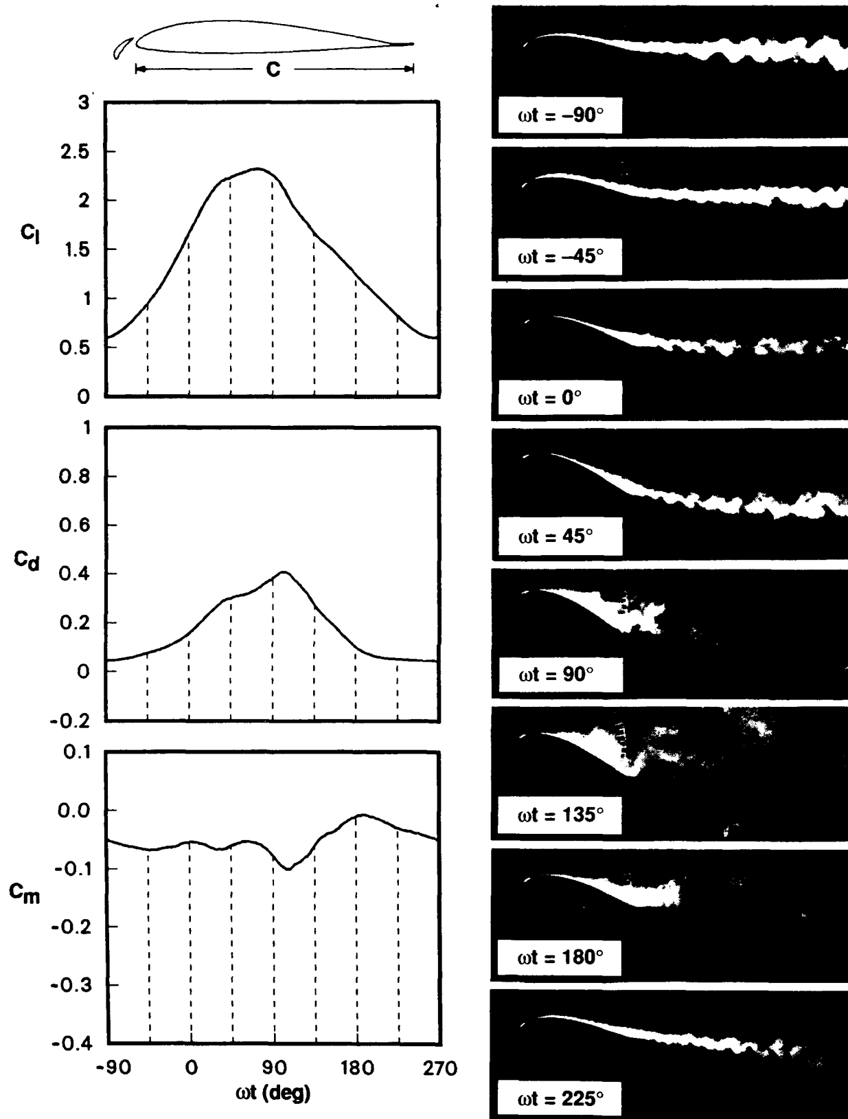
(b) VR-7 airfoil with slat.
