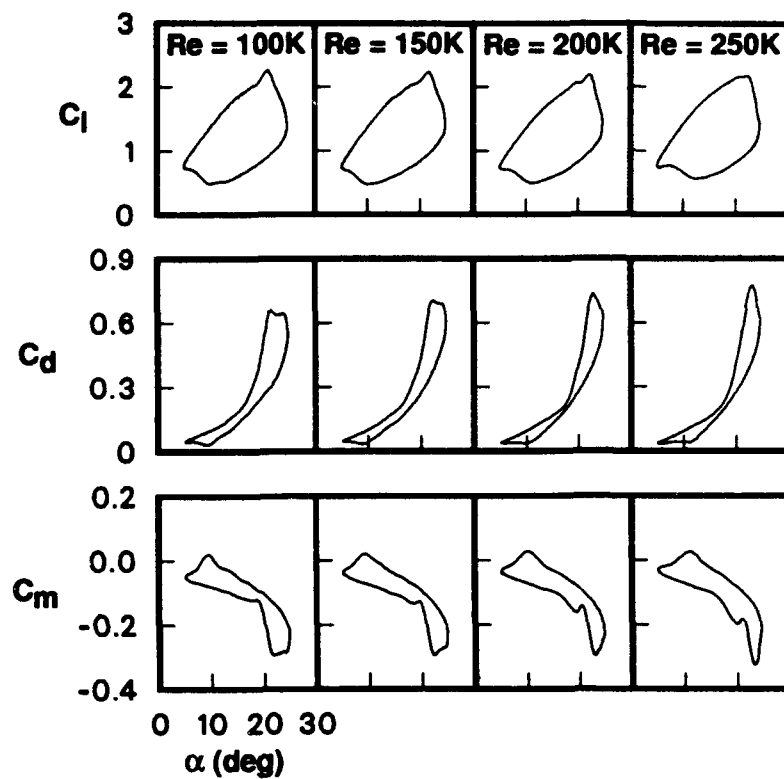
(a) Basic VR-7 airfoil.
