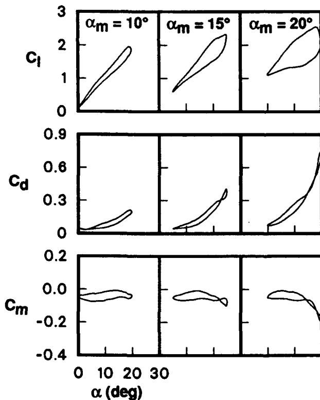
(b) VR-7 airfoil with slat.
