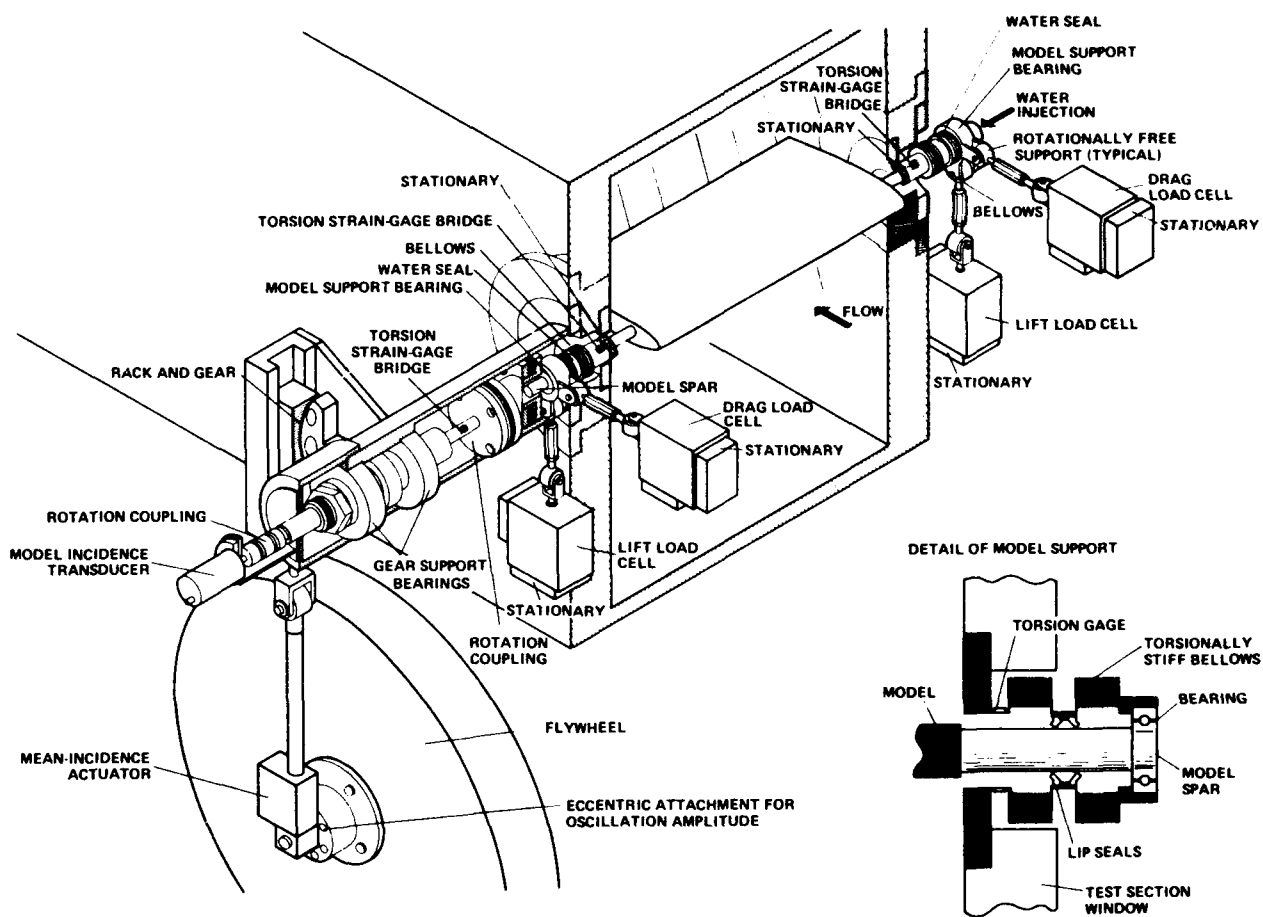
Figure 4. Model installation and balance system for force and moment measurements.
