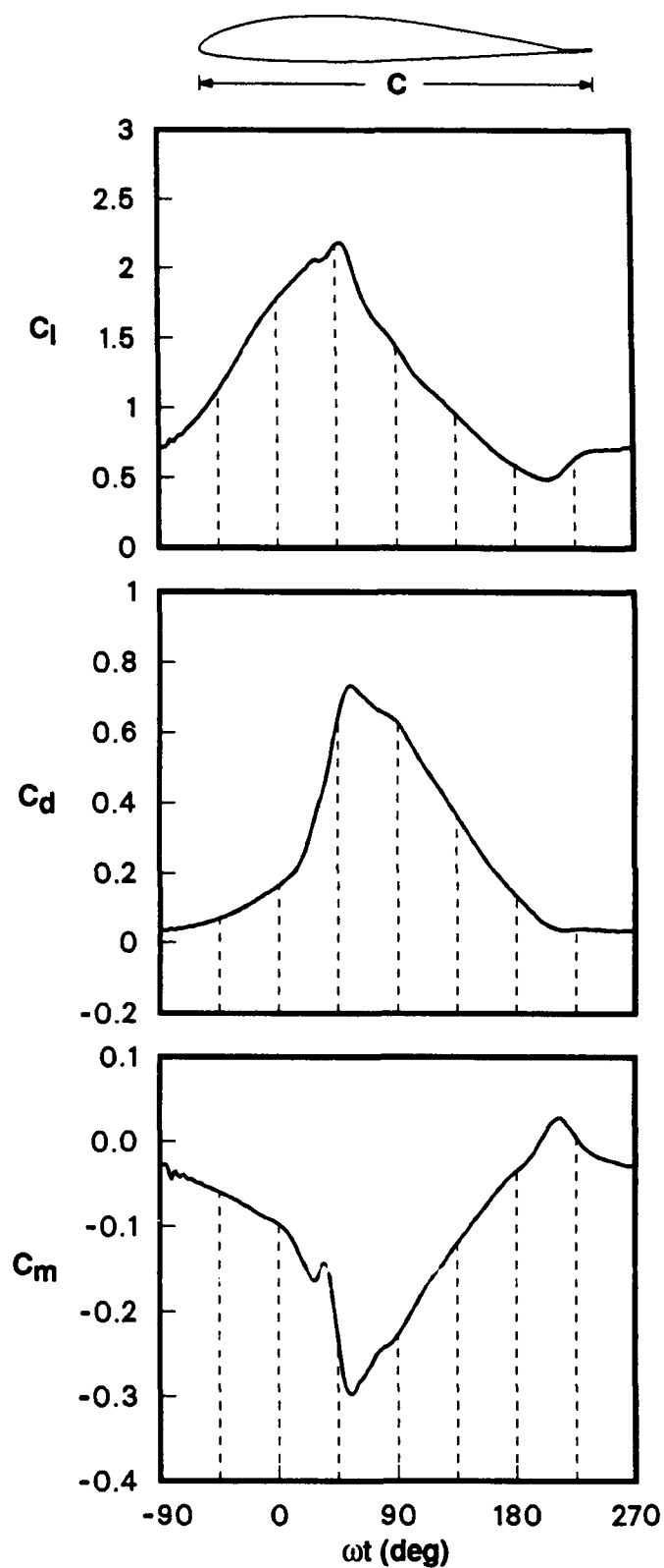
(a) Basic VR-7 airfoil
