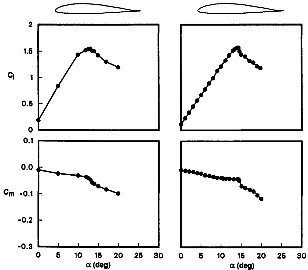
(a) Wind tunnel data (ref. 6) at Re = 1.5 \times 10^6 and M_\infty = 0.11 .
