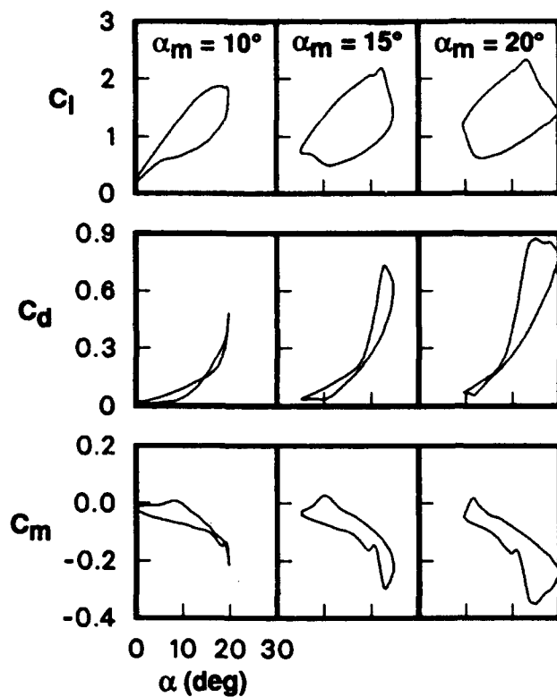
(a) Basic VR-7 airfoil.
