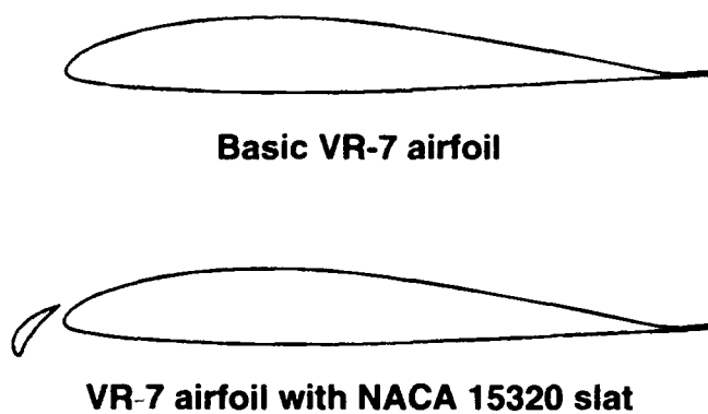
Figure 2. VR-7 airfoil with and without leading-edge slat.
