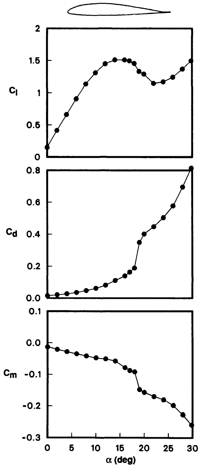
Figure 7. Steady data for the basic NACA 23012 airfoil at Re = 0.2 \times 10^6 .
