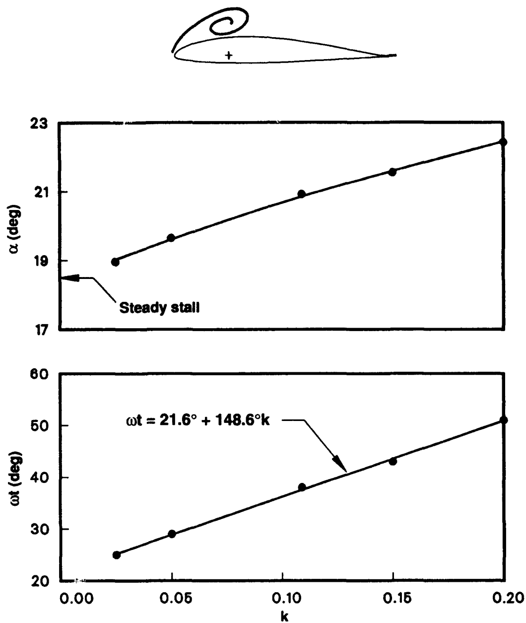
Figure 17. Effect of reduced frequency on the beginning of moment stall for the basic VR-7 airfoil at Re = 200K with \alpha = 15^\circ + 10^\circ \sin(\omega t) .
