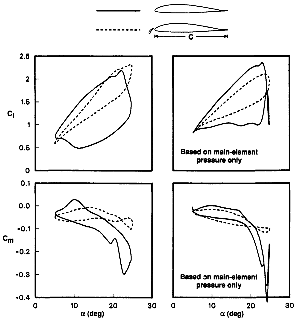
(a) Water tunnel, Re = 2.0 \times 10^5 .
