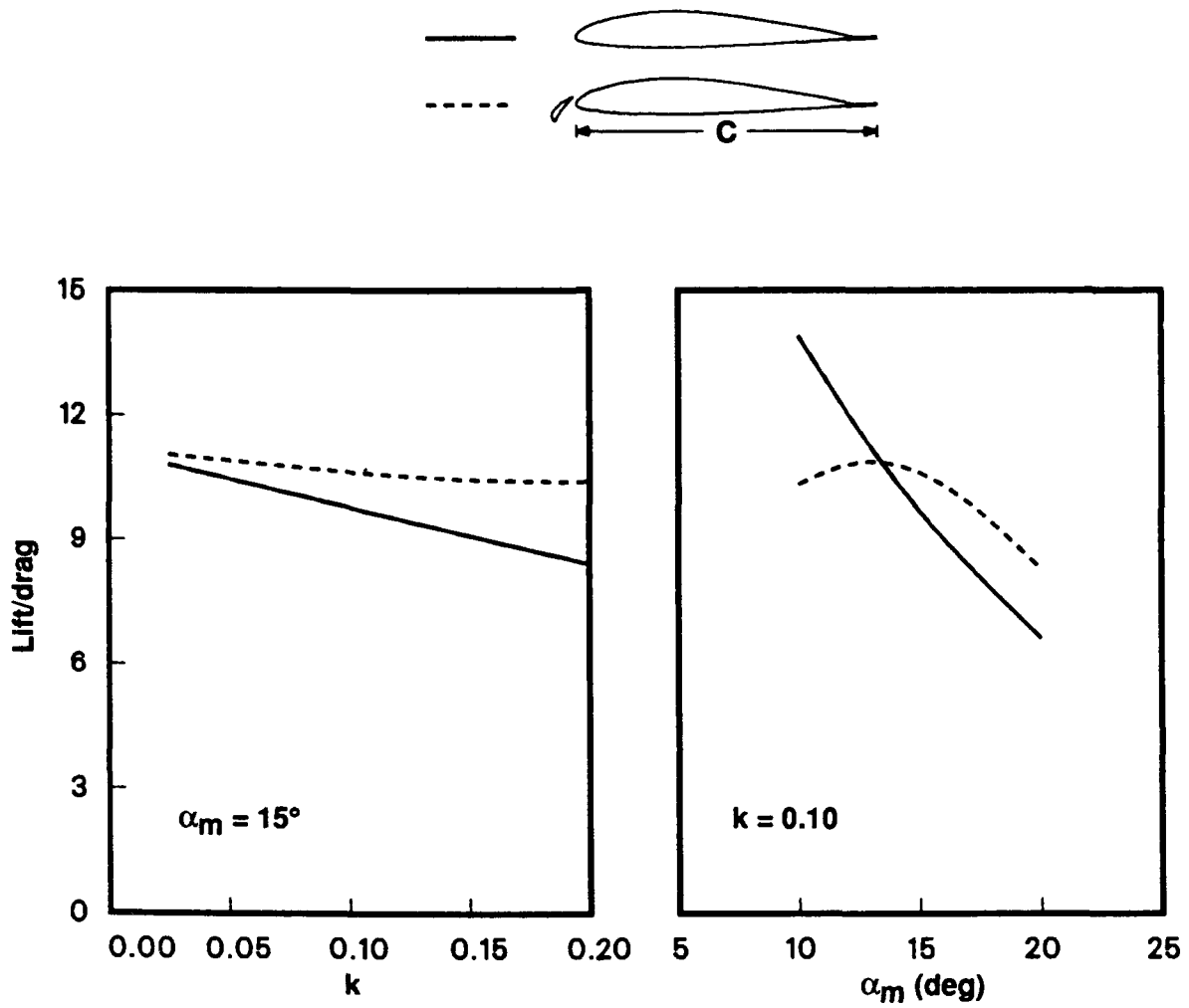
Figure 36. Lift/drag comparison between basic and slatted VR-7 airfoils at Re = 200K for k = 0.025 \rightarrow 0.2 and \alpha_m = 10^\circ \rightarrow 20^\circ with \alpha = \alpha_m + 10^\circ \sin(\omega t) .
