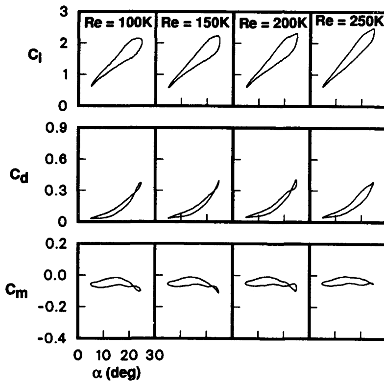
(b) VR-7 airfoil with slat.
