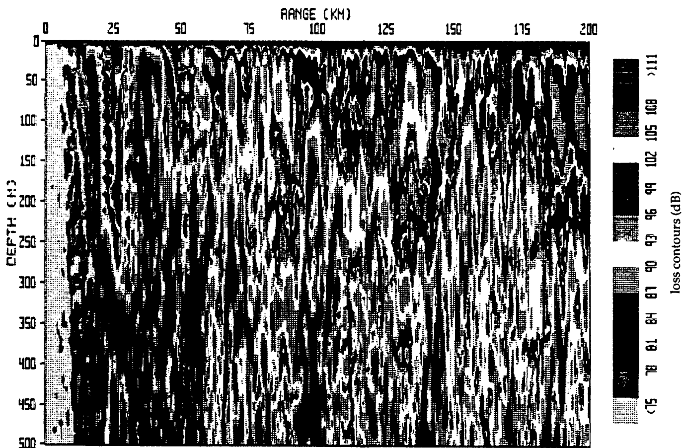
FIGURE 7. PE Propagation loss prediction for an 800m source depth off Kauai. Propagation is approximately uniform on all radials extending from 290° to 70° ref. north.
