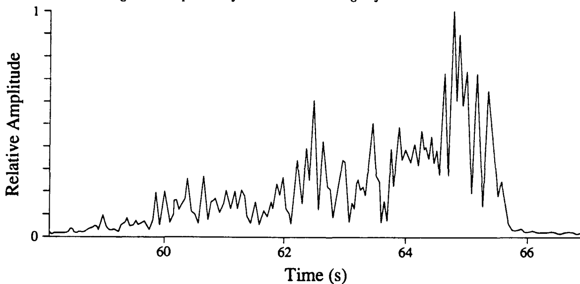
FIGURE 5. Christmas Island (~5 Mm) arrival structure showing complex arrival structures not anticipated for this path.
