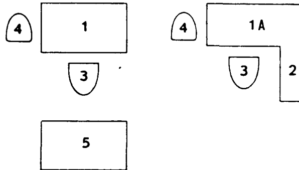
TYPICAL O-1 LAYOUTS
