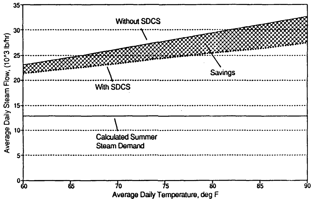
Figure 18. Summer Steam Savings.
