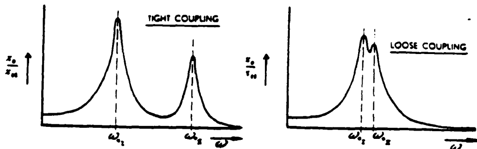
Figure 5.12. Systems with tightly coupled and loosely coupled modes. The spacing of the peaks also indicates that the two modes are loosely coupled. The sharpness of the peaks are also significantly different, indicating their differing damping ratios. The z response is comprised of combinations of modes 2 and 3, the same as the x response. However, the relative contributions of the two modes are opposite.
