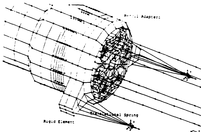
Figure 3.10. Recoil Adapters.
