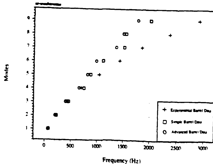
Figure 4.20. Comparison of the model and actual barrels.
