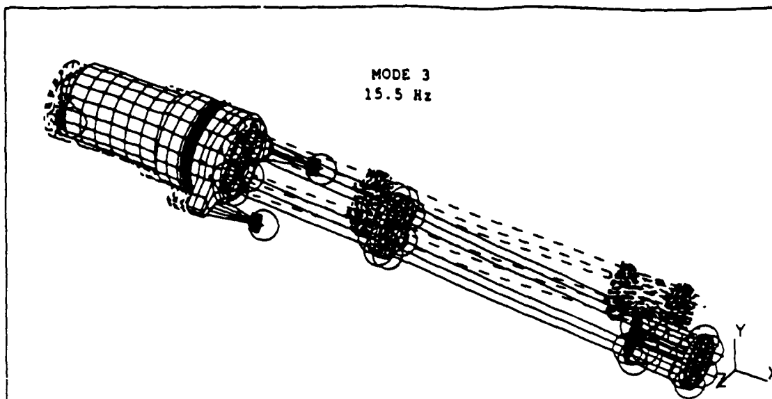
Figure 4.5. Isometric view of MODE 3.
