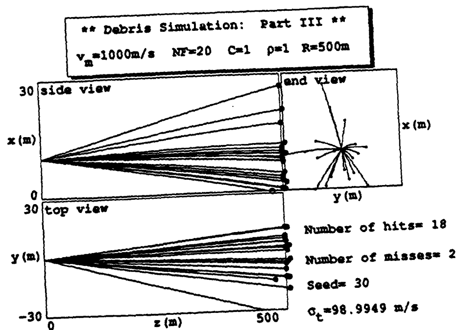
Figure 1.7. Ballistic missile fragment trajectories.
