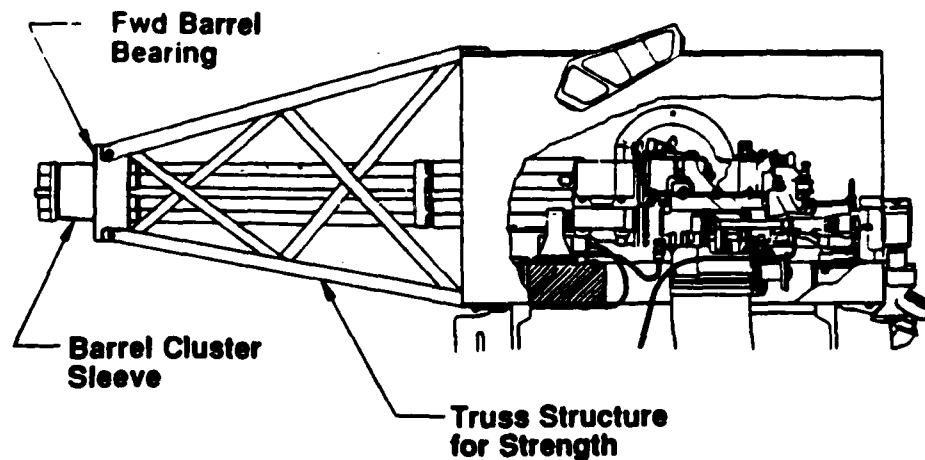
Figure 6.1. Muzzle restraint.
