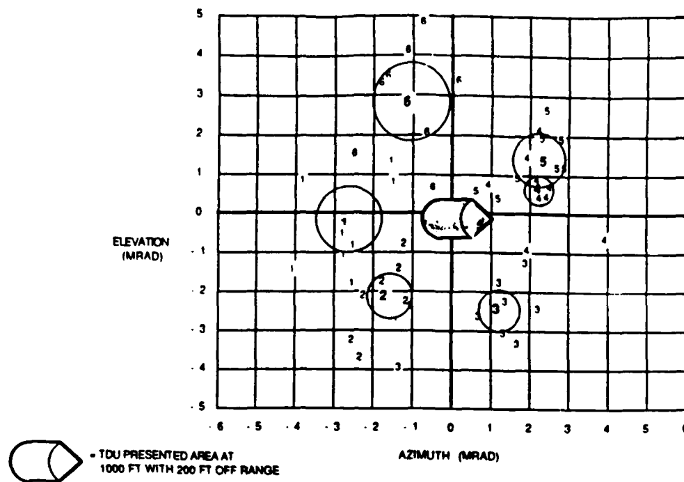
Figure 1.6. Dispersion Pattern.
