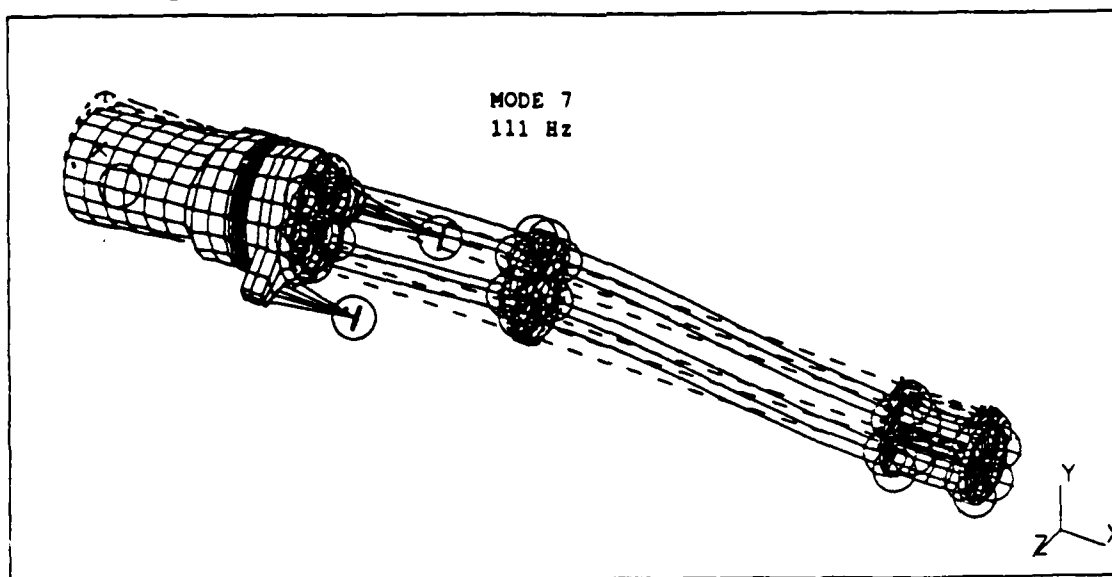
Figure 4.9. Isometric view of MODE 7.
