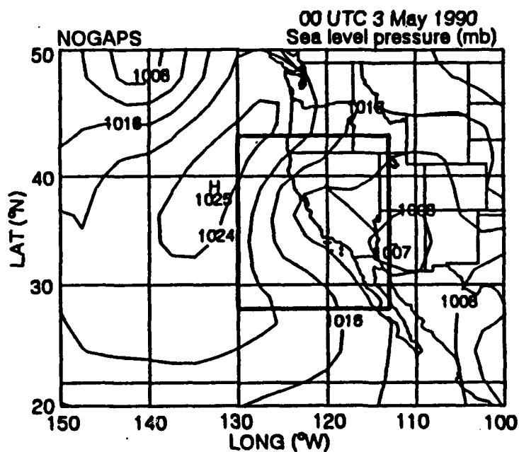
Figure 6C 0000 UTC 03 May 1990 NOGAPS Sea Level Pressure Analysis
