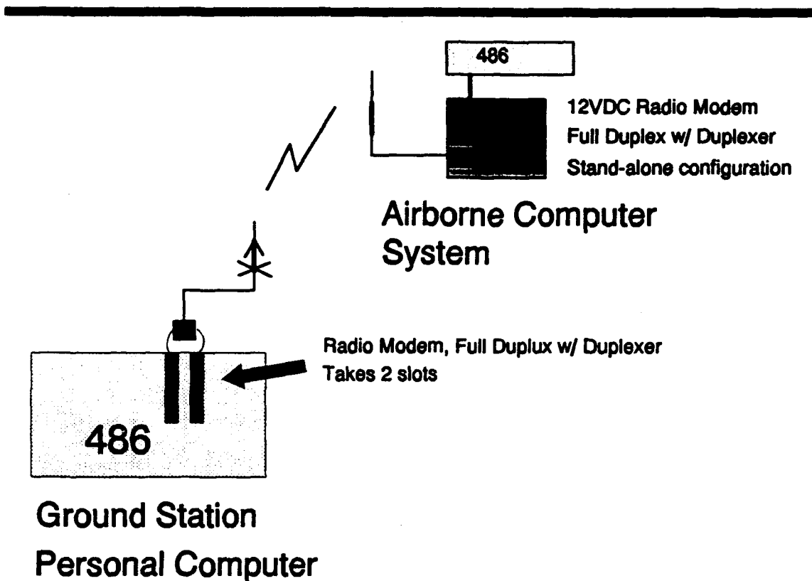
Figure 10 Typical radio modem configuration.
