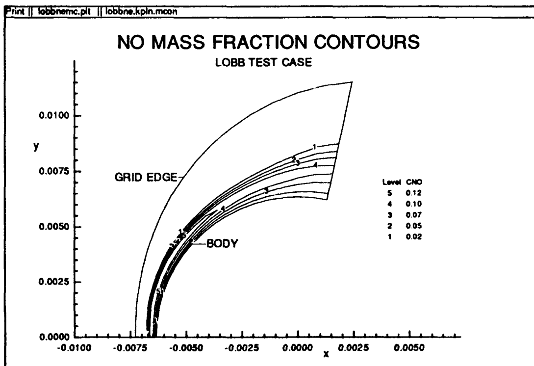
Fig.4 NO mass fractions, Lobb test case.
