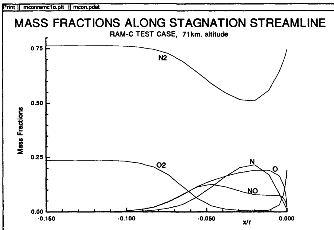
Fig.12 Stagnation streamline mass fractions, RAM-C II test case.
