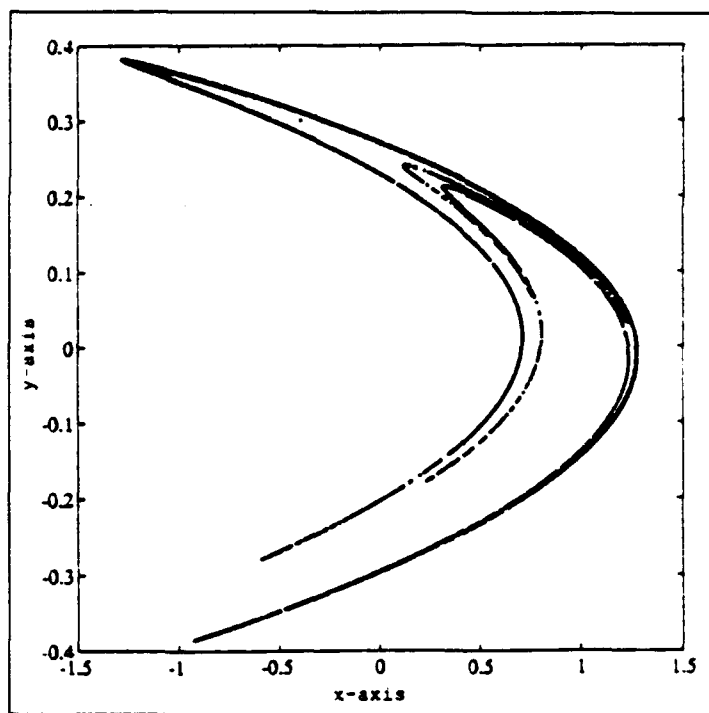
Figure 1 Hénon attractor
