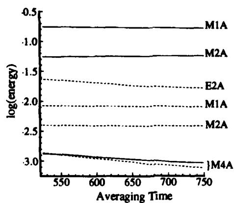
Figure 3. Coherent energies: - - - kinetic, - - - - magnetic.
