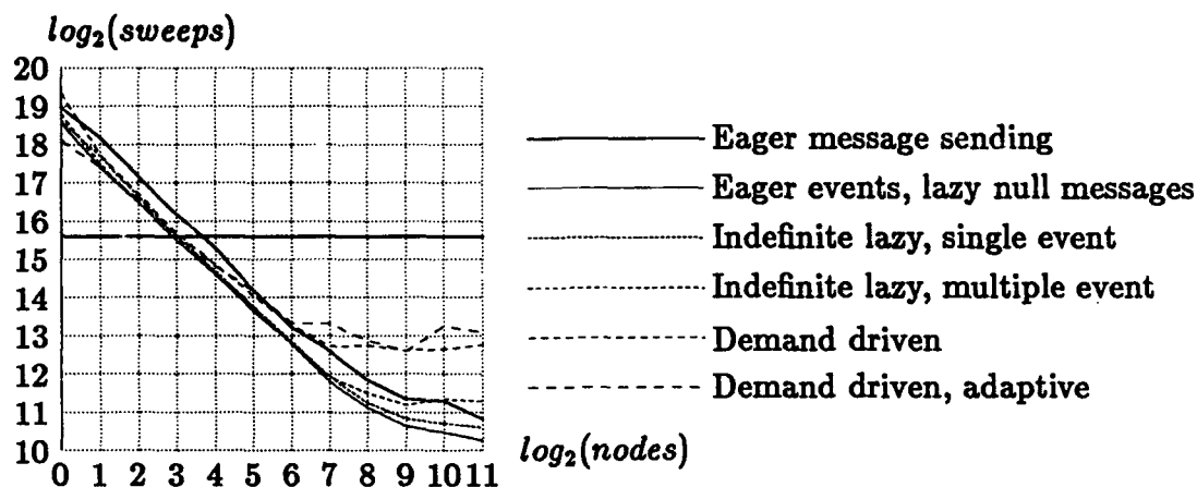
Fig 1: A 1376-gate multiplier, emulation mode
