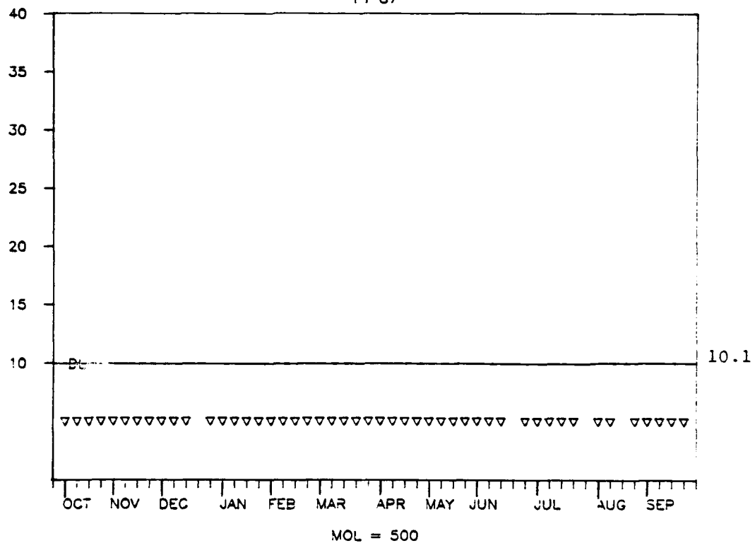
Figure 12. FY87 Diisopropylmethylphosphonate
