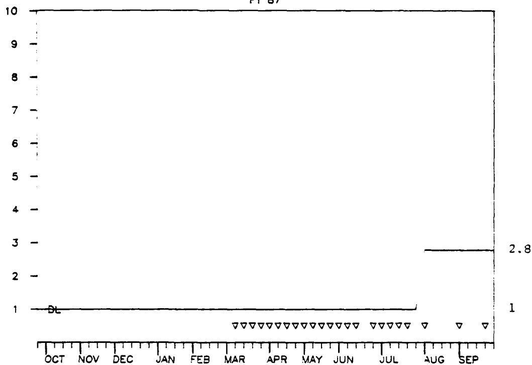
Figure 9 . FY87 Tetrachloroethylene
