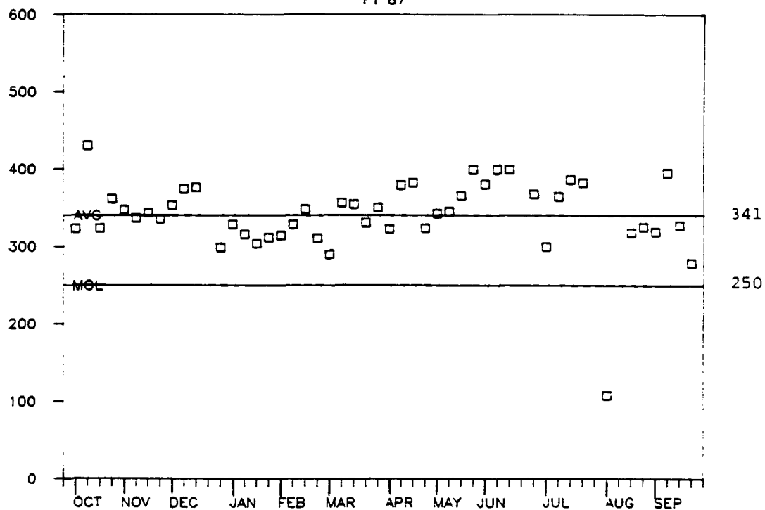
Figure 16. FY87 Chloride
