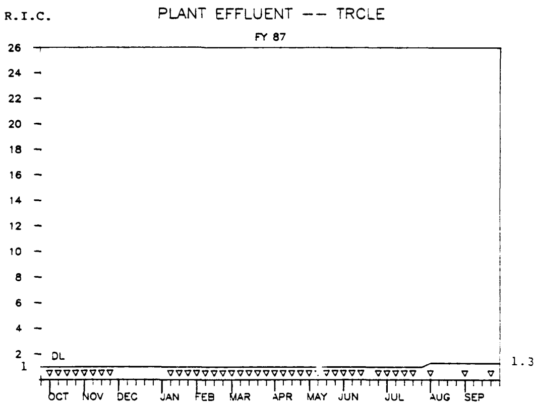
Figure 8 . FY87 Trichloroethylene
