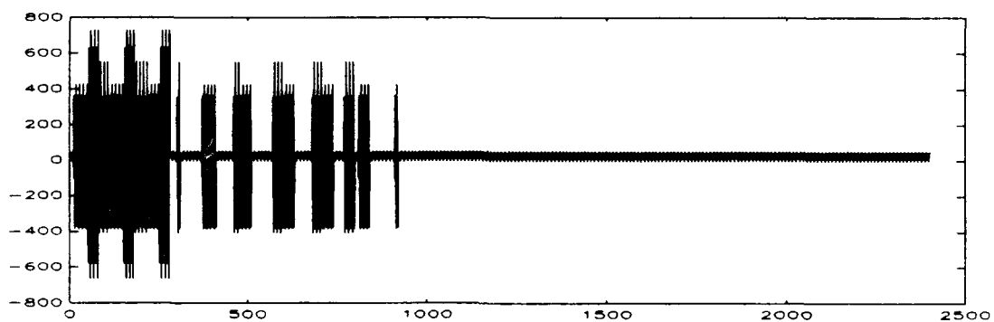
Figure 4.12 Transient Signal Coded by DVQ at 1.0 bps, SNR = 3.9 dB.
