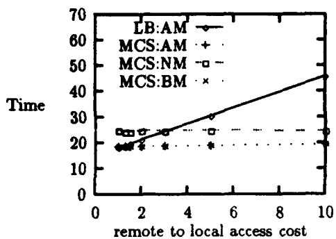
Uniform Execution Times
