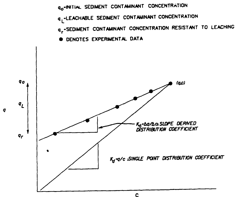
Figure V-27. Desorption Isotherm Illustrating Constant Partitioning
