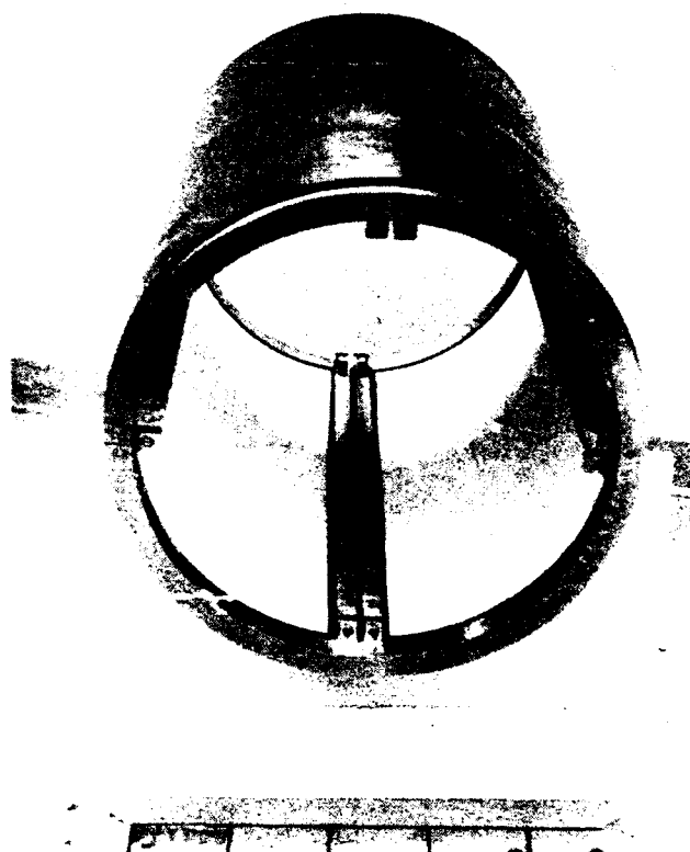
Figure 3. Internal mounts for payload platform inside the 20-inch OD alumina-ceramic cylinders.
