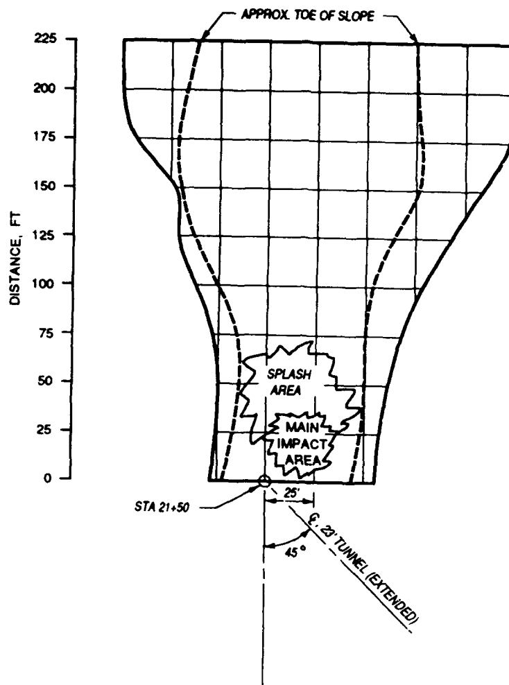
PLAN VIEW OF EXIT CHANNEL TYPE 7 DESIGN EXIT STRUCTURE POOL EL 925 BOTH GATES OPEN FULL DISCHARGE 1,500 cfs (ESTIMATED) n = 0.018
