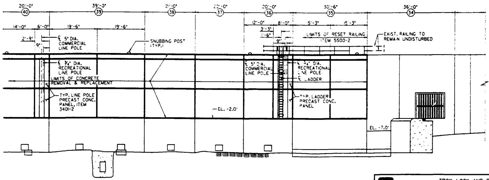
WEST LOCK WALL - ELEVATION SCALE: 1" = 20'-0"
