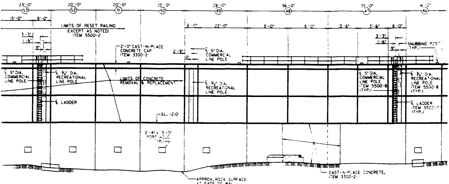
WEST LOCK WALL - ELEVATION SCALE: 1" = 20'-0"
