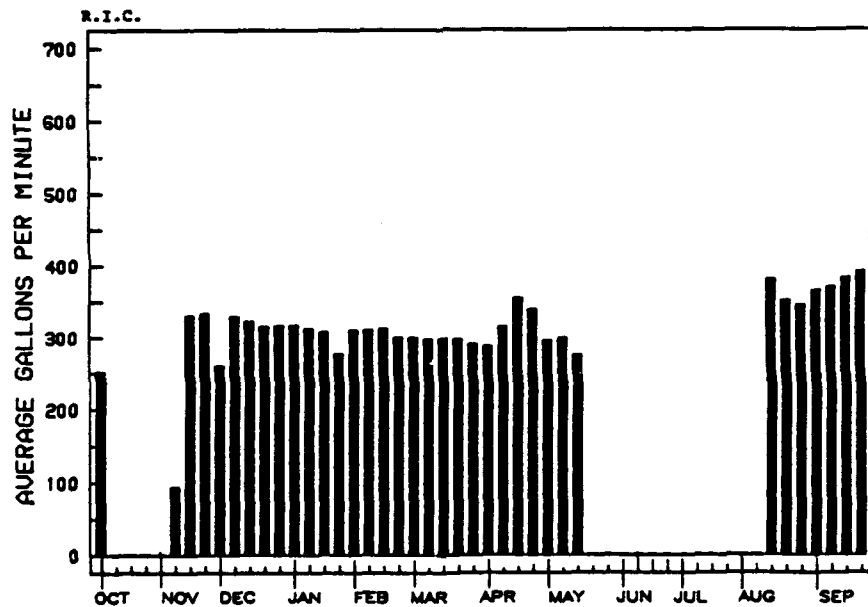
Figure 3. Adsorber 2 flow rate during FY88.
