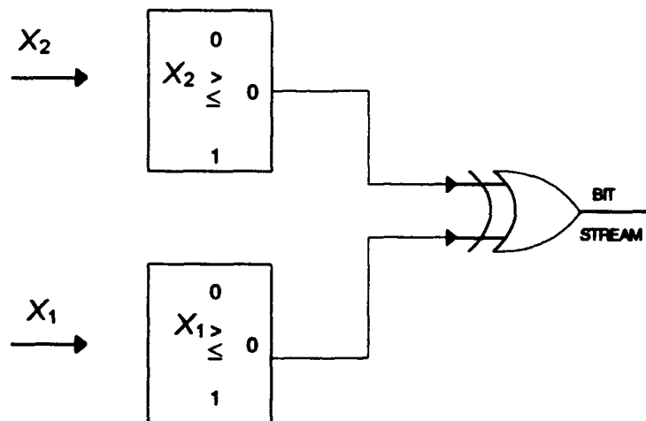
Figure 16. Decision Logic for MSK Receiver.
