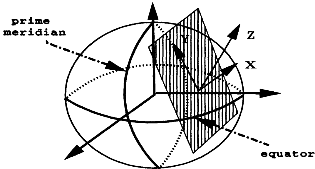
Figure 2.3: Tangent Plane Coordinate System
