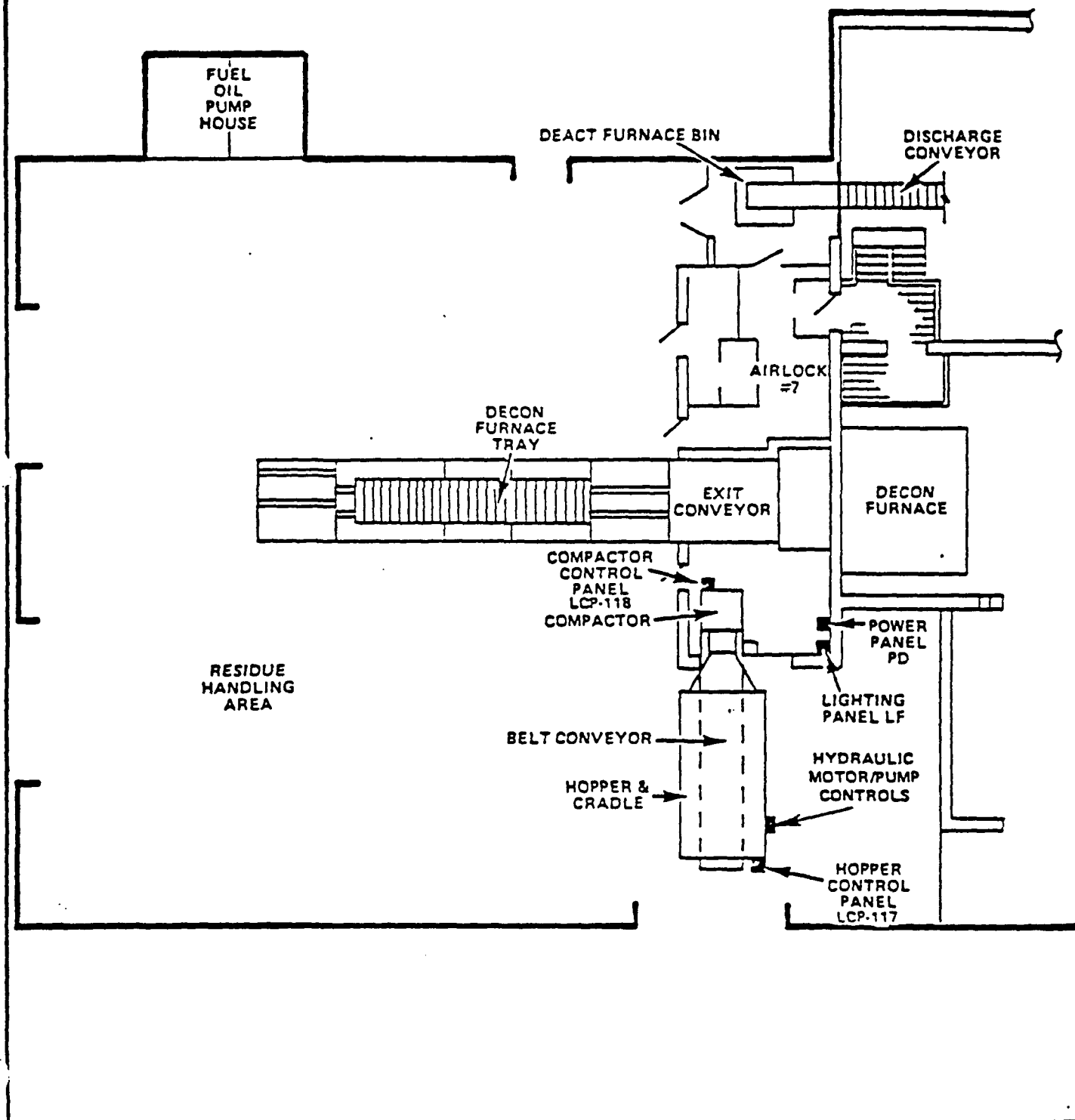
Fig. 14. RESIDUE HANDLING EQUIPMENT LOCATION
