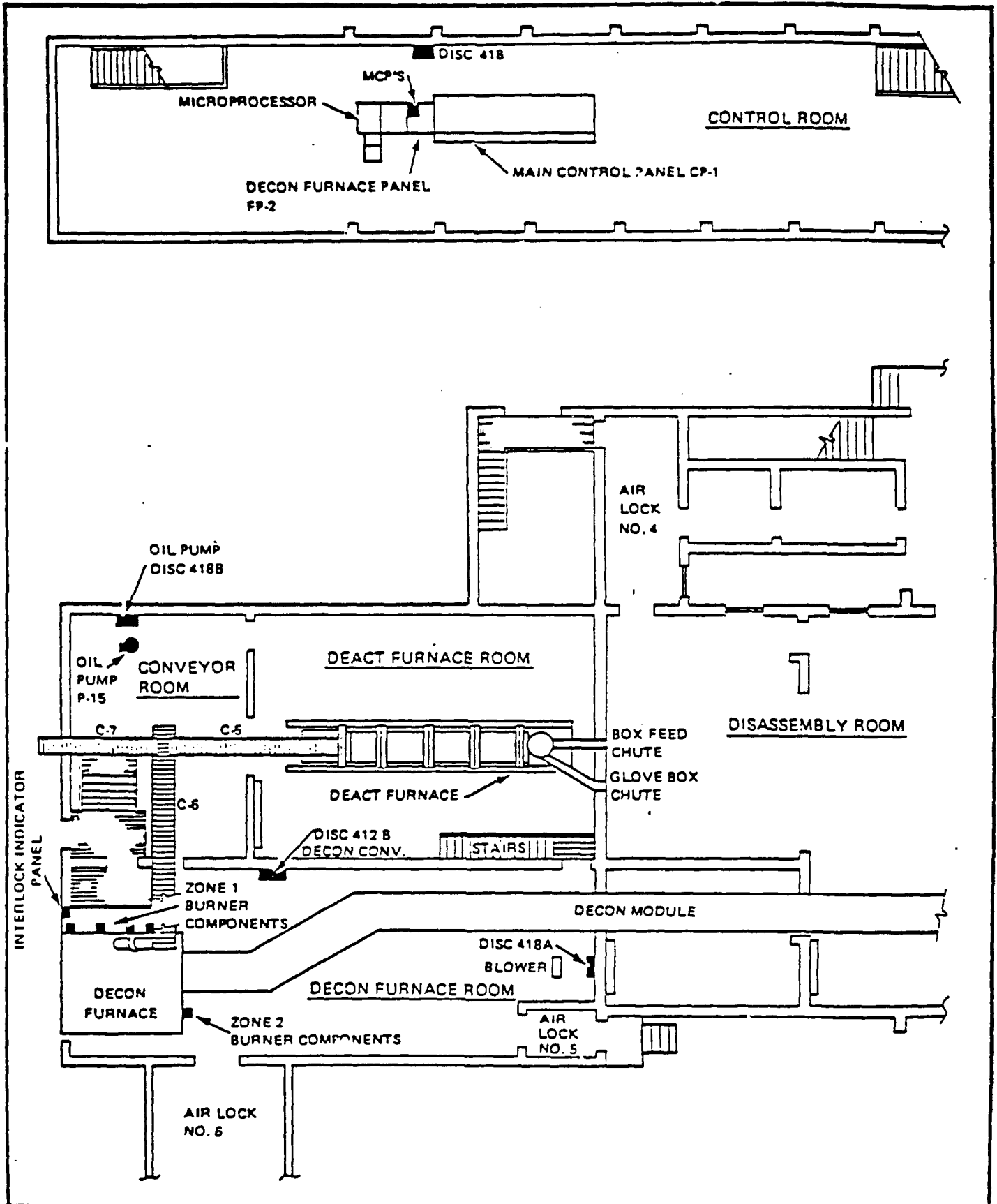
Fig. 12. DECON FURNACE EQUIPMENT LOCATION
