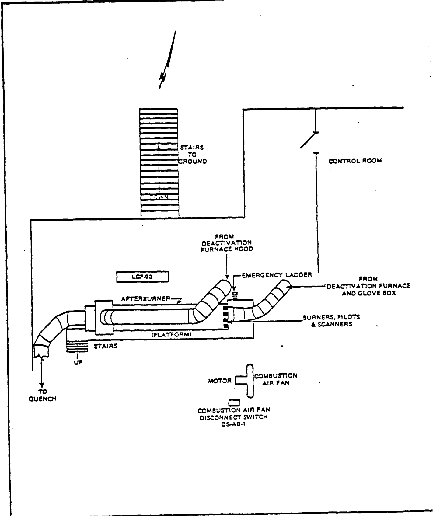
Fig. 17. - AFTERBURNER EQUIPMENT LOCATION (NORTHWEST ROOF CORNER)
