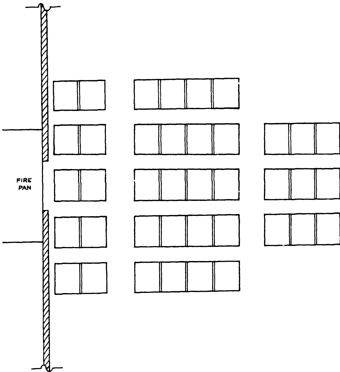
FIGURE 2. SEAT CONFIGURATION
