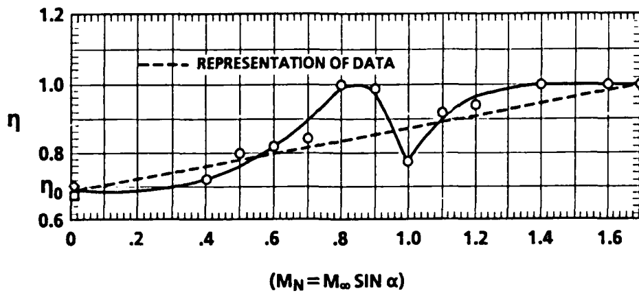
FIGURE 3-11A. COMPRESSIBILITY EFFECTS ON CROSSFLOW DRAG PROPORTIONALITY FACTOR
