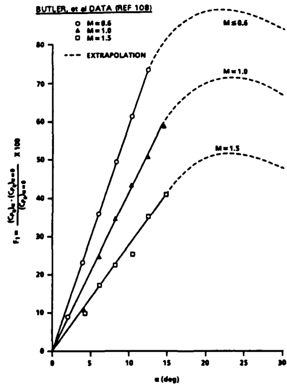
B. ( M_\infty < 2 )
