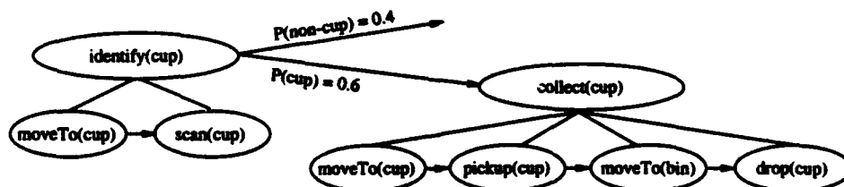
Figure 2: Cup Collection Plan.
