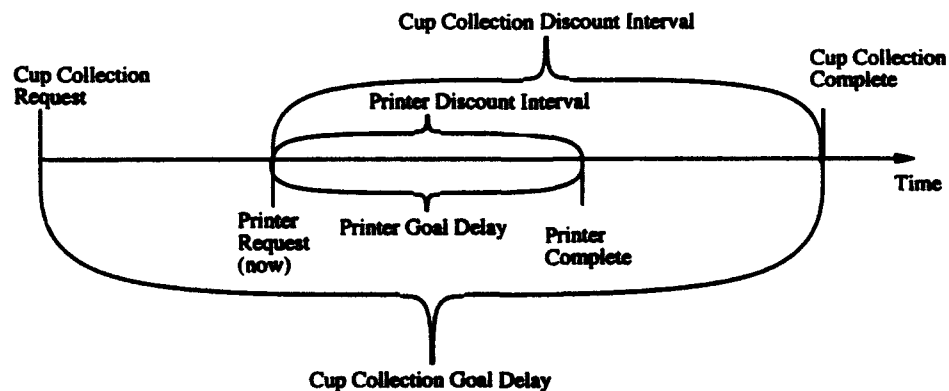
Figure 8: Time Line for Suspending Cup Collection.
