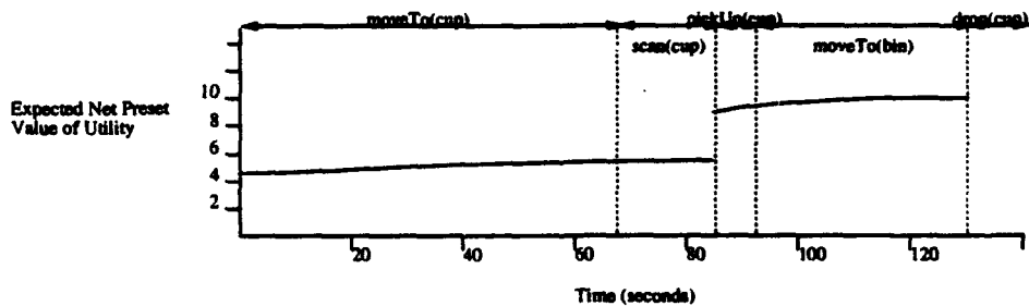
Figure 10: Cup Collection Utility Versus Time.
