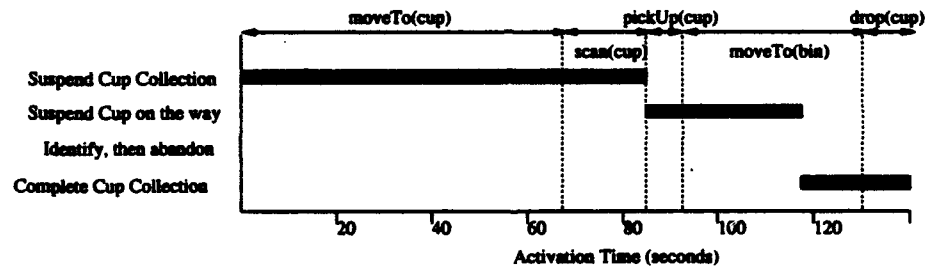
Figure 7: Best Goal Ordering versus Activation Time. (Cup Collection)
