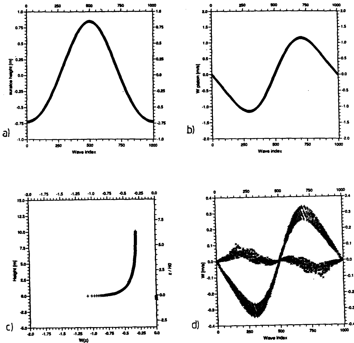
Figure 3.6: Parameters for the wind field W(x,z) a) Height of wave surface versus x -grid index b) Piston velocity versus x -grid index c) Example of local profile of vertical wind component d) Vertical wind component distribution over the wave at 10 m (see text)
