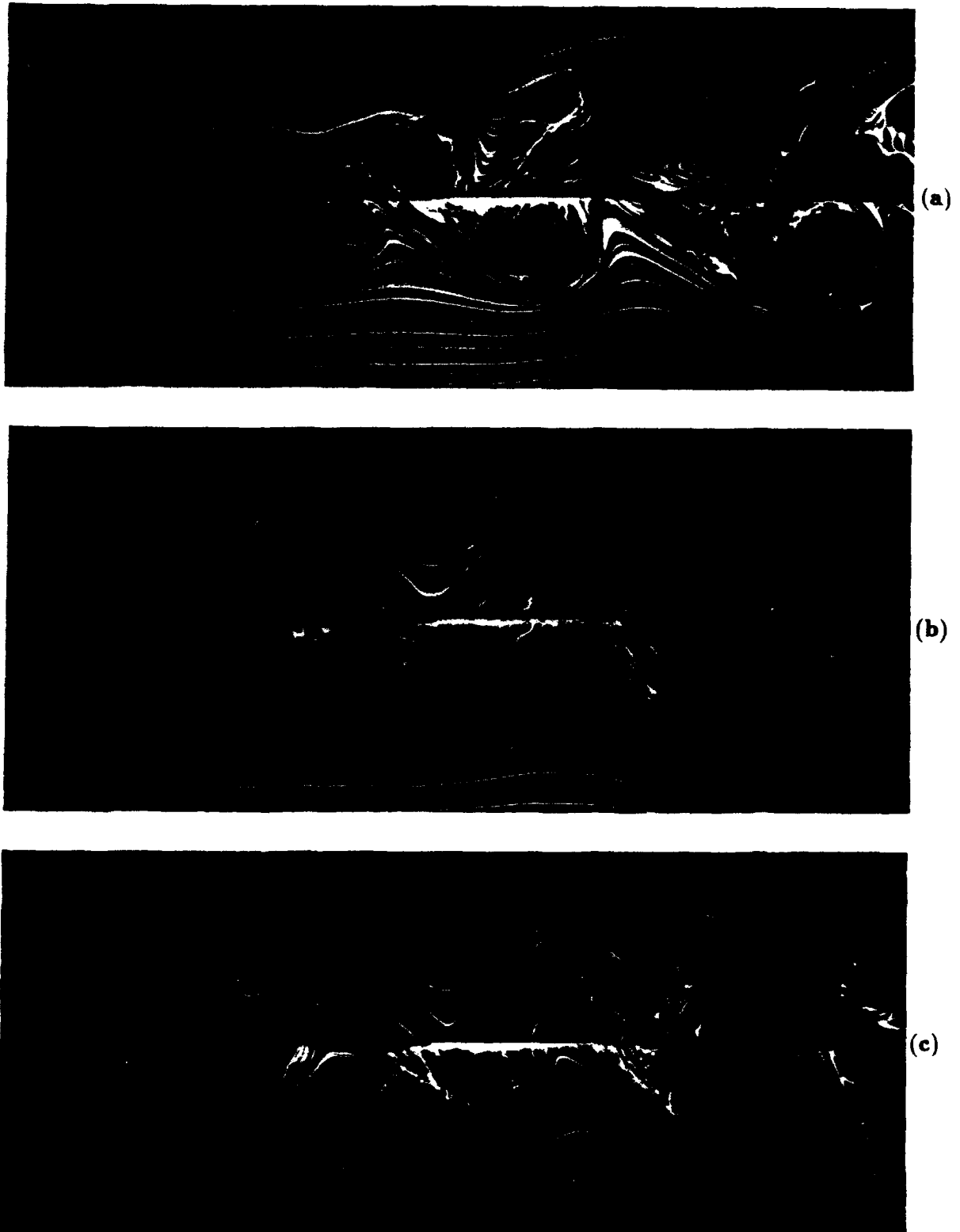
FIG. 3.4 Smoke wire visualization of the flow past a circular cylinder with a permeable splitter plate, \sigma = 0.22 : (a) Re = 2500 , (b) Re = 5500 , (c) Re = 8000 .
