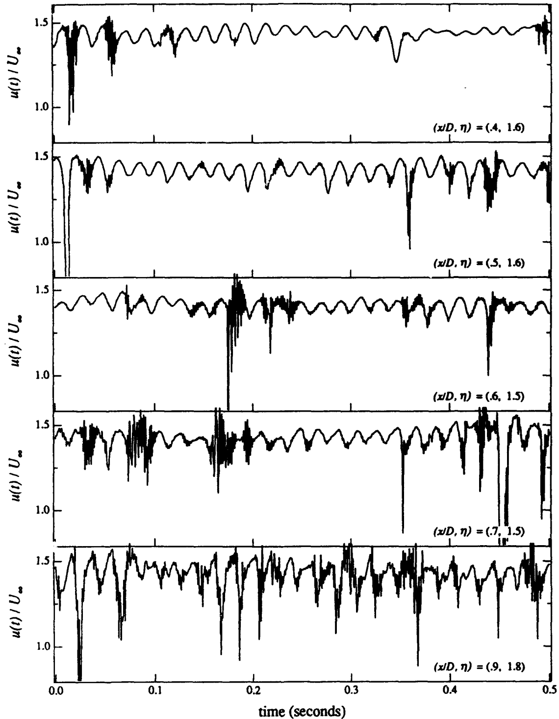
FIG. 5.6 Shear layer velocity traces showing the evolution of the shear layer instability with downstream position. Each trace in the figure corresponds to a different downstream location. Downstream location x/D and normalized transverse shear layer coordinate \eta are shown on each trace (figure continues on next page).
