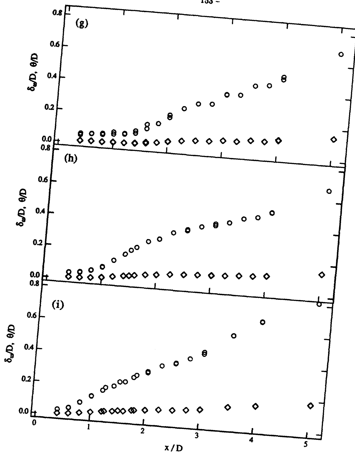
FIG. 5.4 cont. (g) \sigma = 0.65, Re = 4900 , (h) \sigma = 0.65, Re = 9400 , (i) \sigma = 0.65, Re = 15200 .
