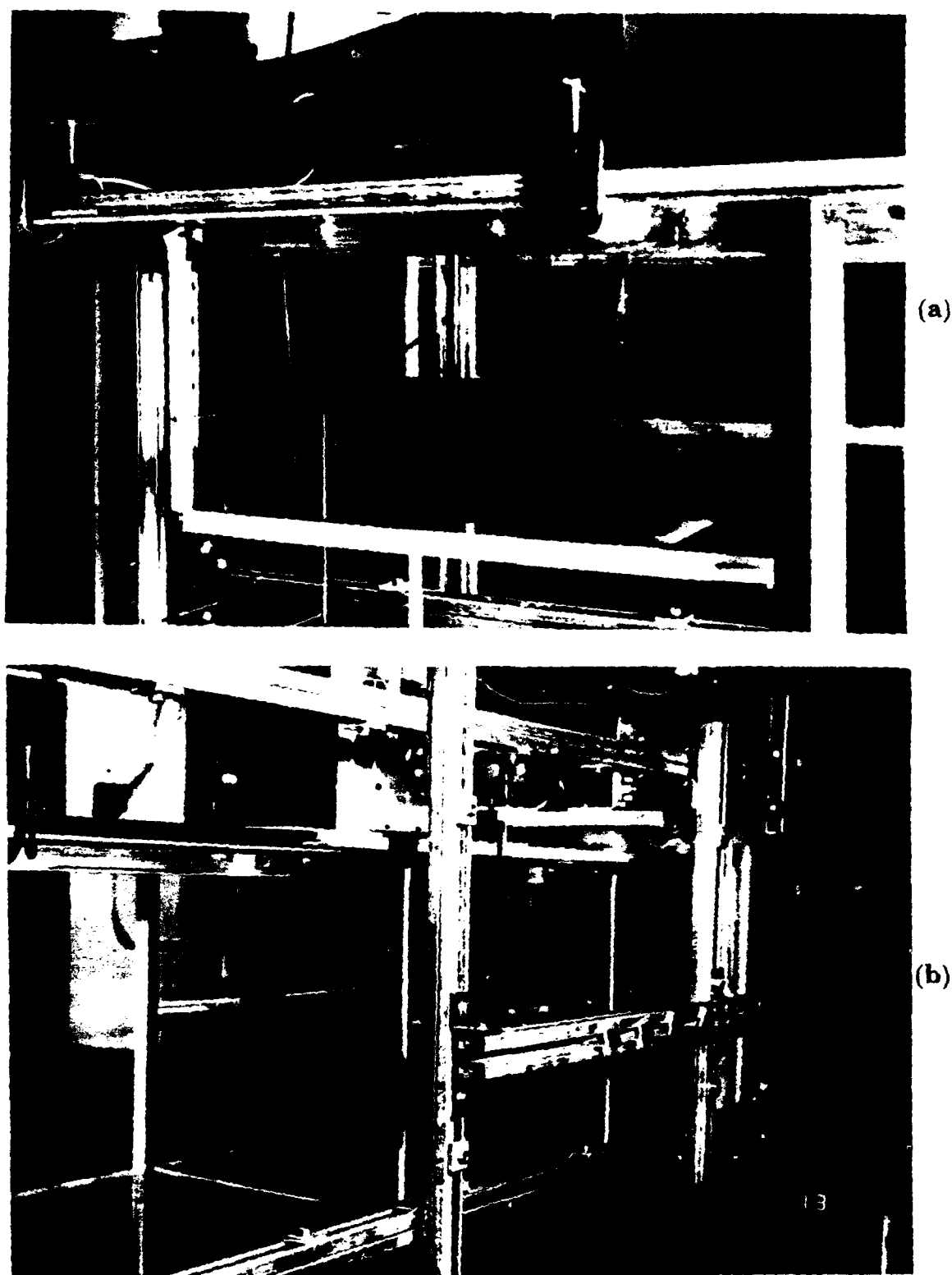
FIG. 2.1 Photos of the assembled test section with the cylinder, endplates, and a permeable splitter plate installed. (a) Front view, (b) Rear view showing the frame used for tensioning the permeable splitter plates.
