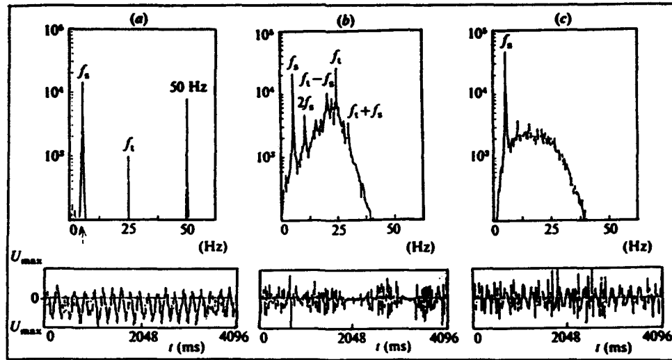
FIGURE 8. Power spectra and traces in the shear layer: Y/D = 0.625 , Re = 2660 . (a) X/D = 0.125 ; (b) 1.375; (c) 3.525 (arbitrary scales).
