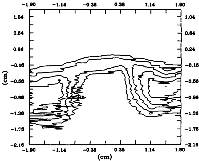
Figure 48.b. Blade 5, Velocity Contours, 1.37c
