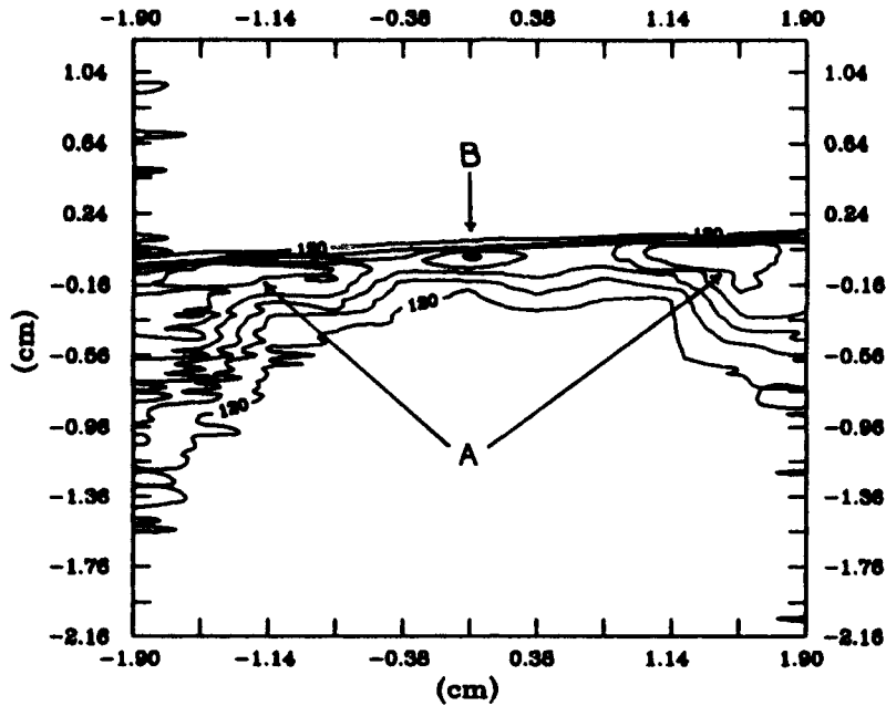
Figure 25.a. Blade 4, Velocity Contours, 0.05c
