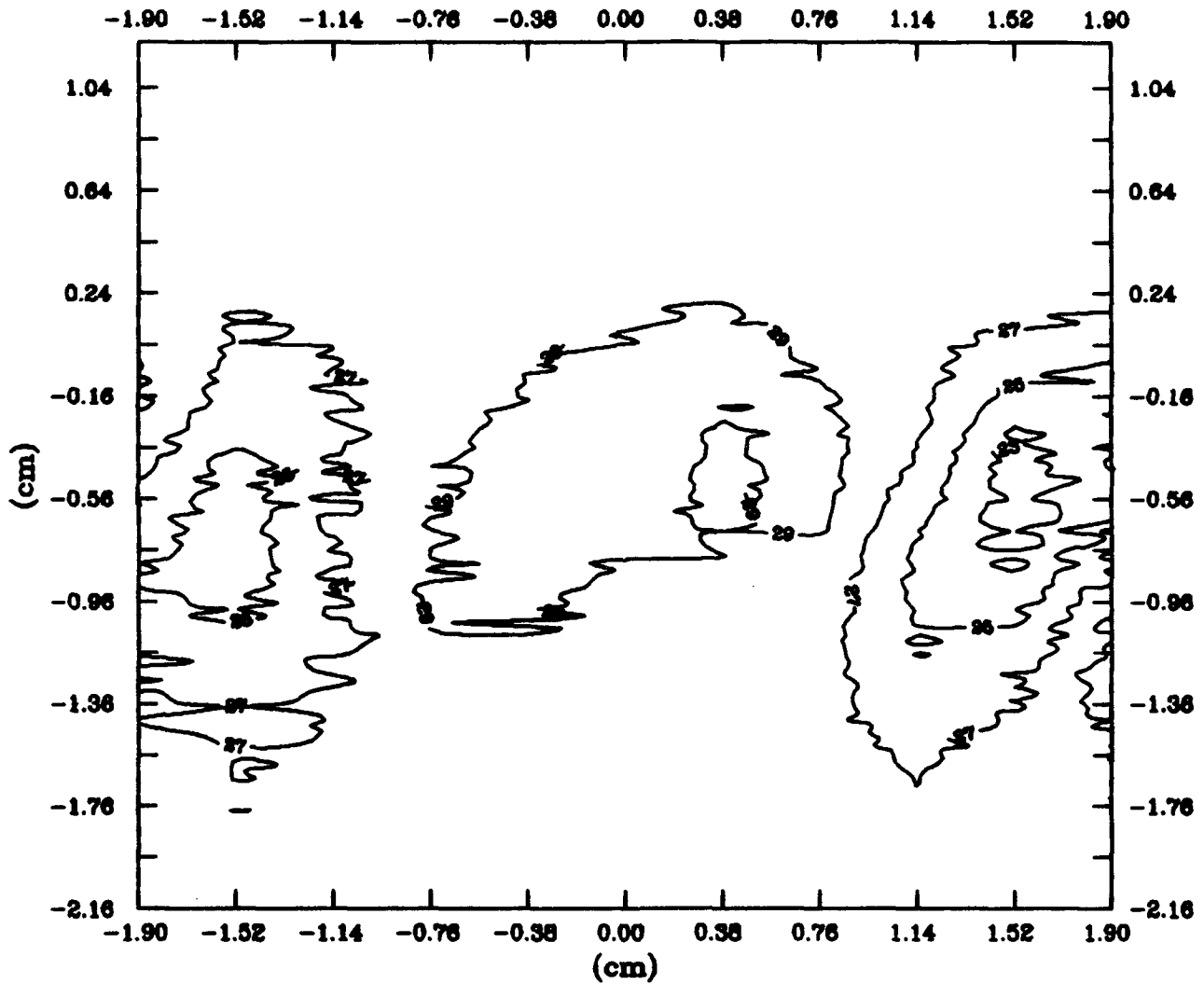
Turning Angle Contours, Blade 4, 1.37c
