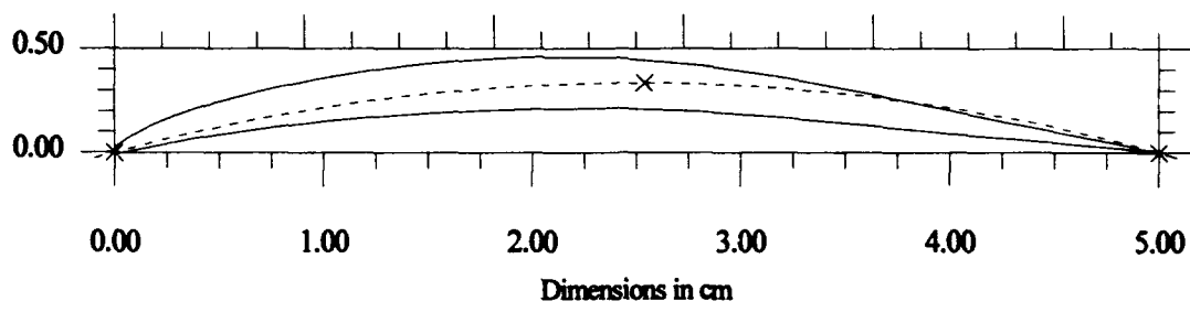
Figure 44. Blade Profile with Circular Arc
