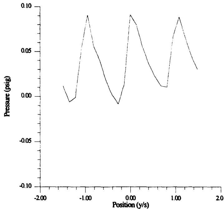
Figure 17. Exit Periodicity (23 ports)
