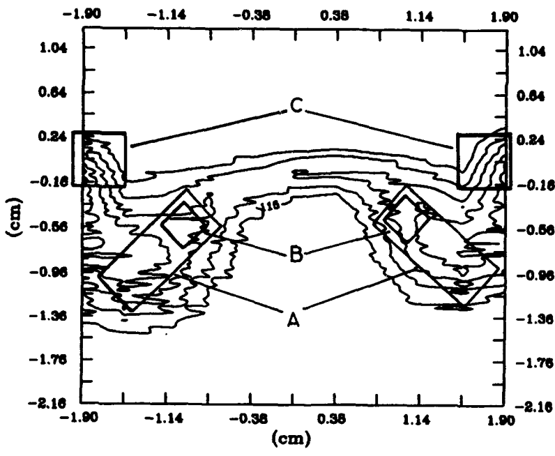
Figure 22.b. Straight Blades, Velocity Contours, 1.37c
