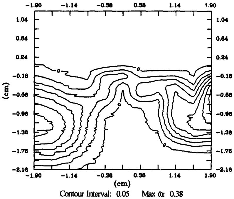
Figure 31.b. Blade 3, \omega Contours, 1.37c
