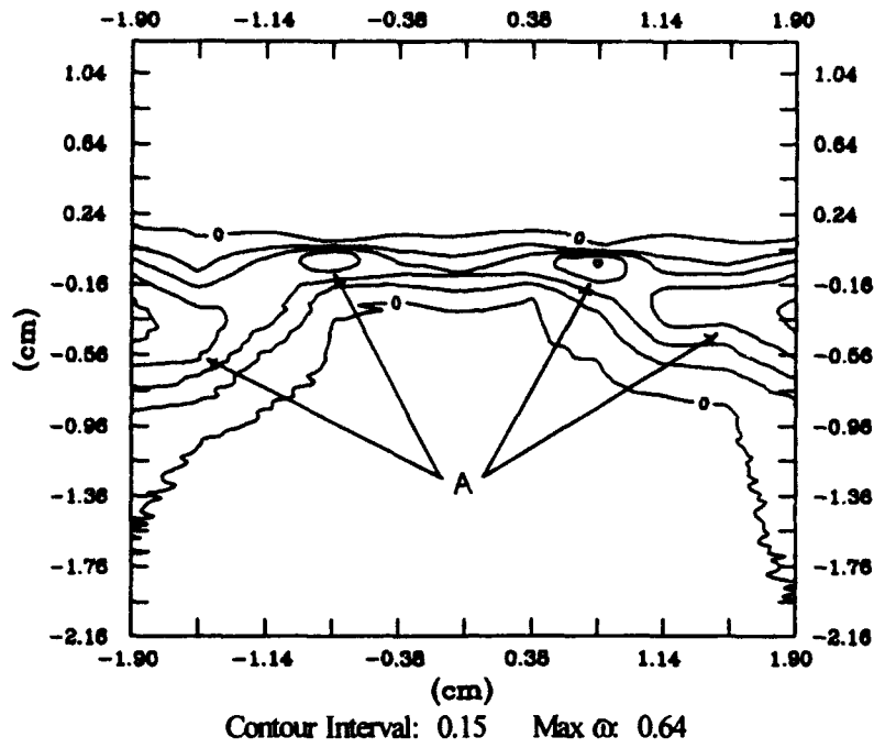
Figure 30.a. Blade 2, \omega Contours, 0.05c
