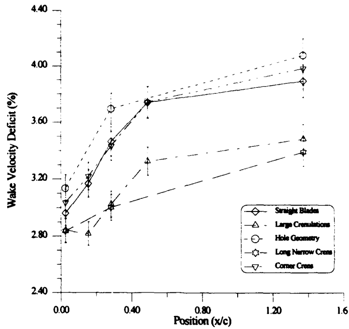
Figure 49. Wake Velocity Deficit (including corner crenulations)
