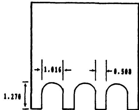
Figure 2.b. Large Crenulation Geometry (Blade 2)
