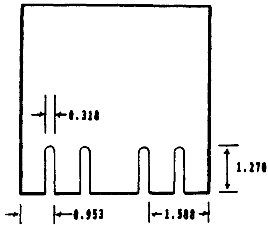
Figure 42.a. Design 1
