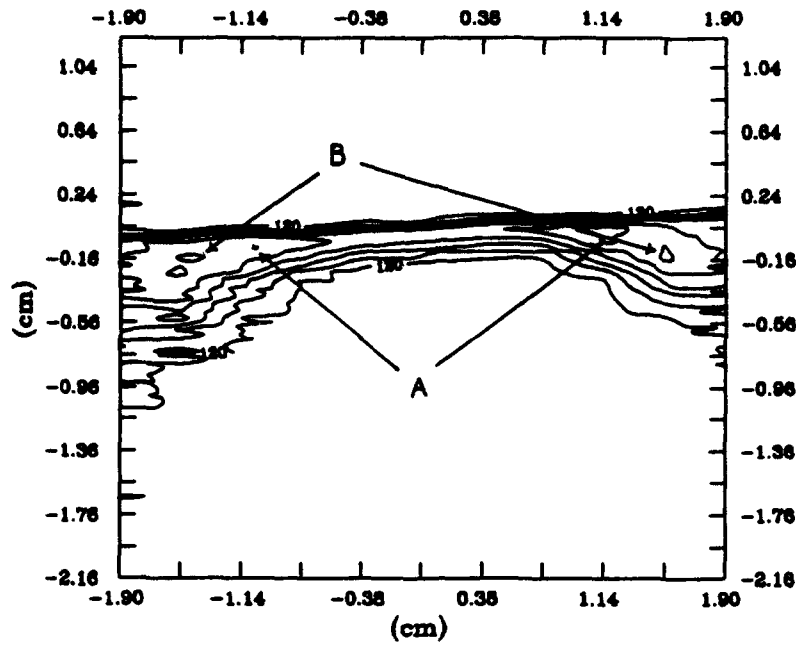
Figure 22.a. Straight Blades, Velocity Contours, 0.05c
