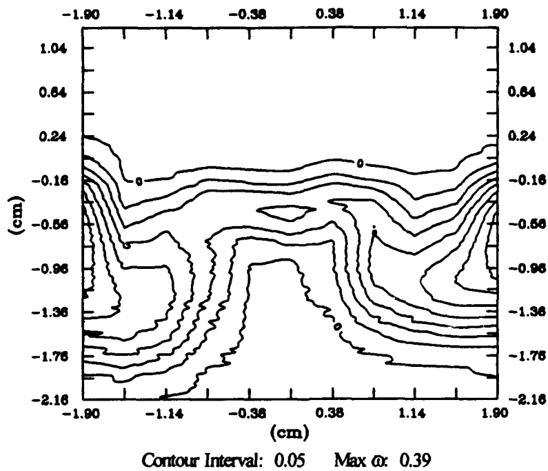
Figure 30.b. Blade 2, \omega Contours, 1.37c
