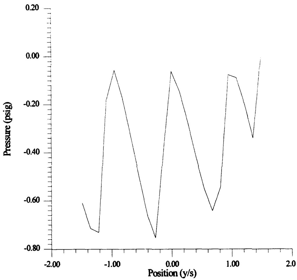
Figure 14. Inlet Periodicity, i = 12.44^\circ
