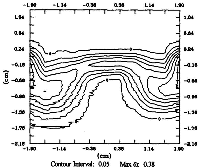
Figure 29.b. Straight Blades, \alpha Contours, 1.37c
