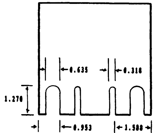
Figure 42.b. Design 2
