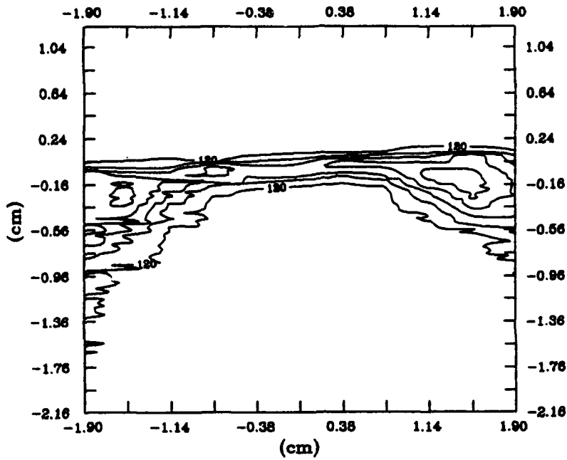
Figure 48.a. Blade 5, Velocity Contours, 0.05c
