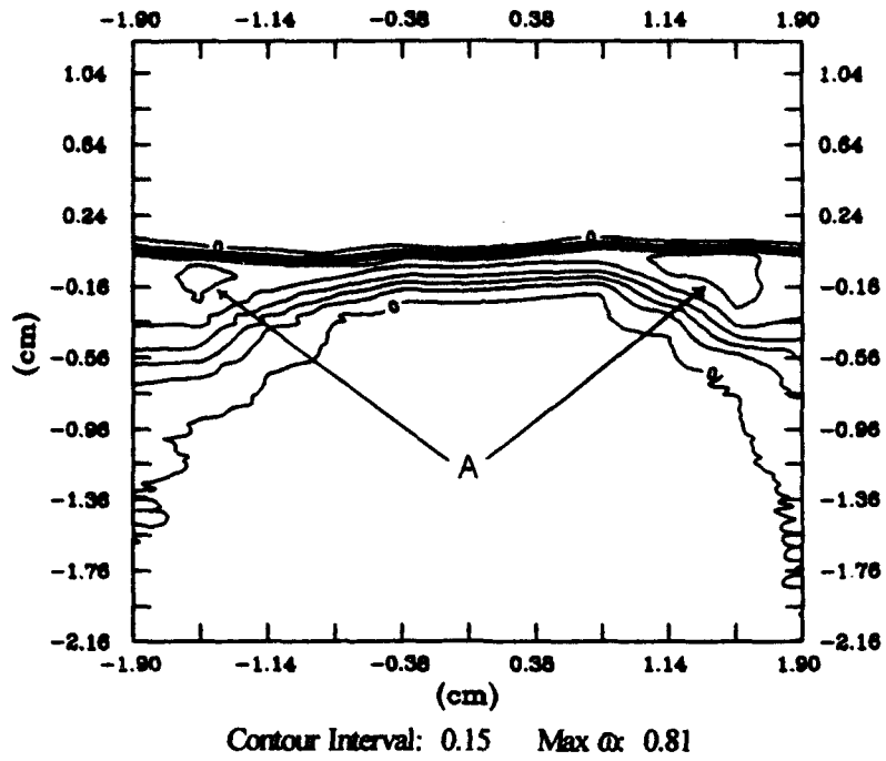
Figure 29.a. Straight Blades, \alpha Contours, 0.05c
