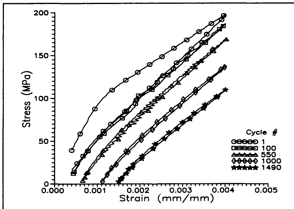
Figure B.2 90° Lamina \sigma - \epsilon History, \epsilon_{\max} = .4\%
