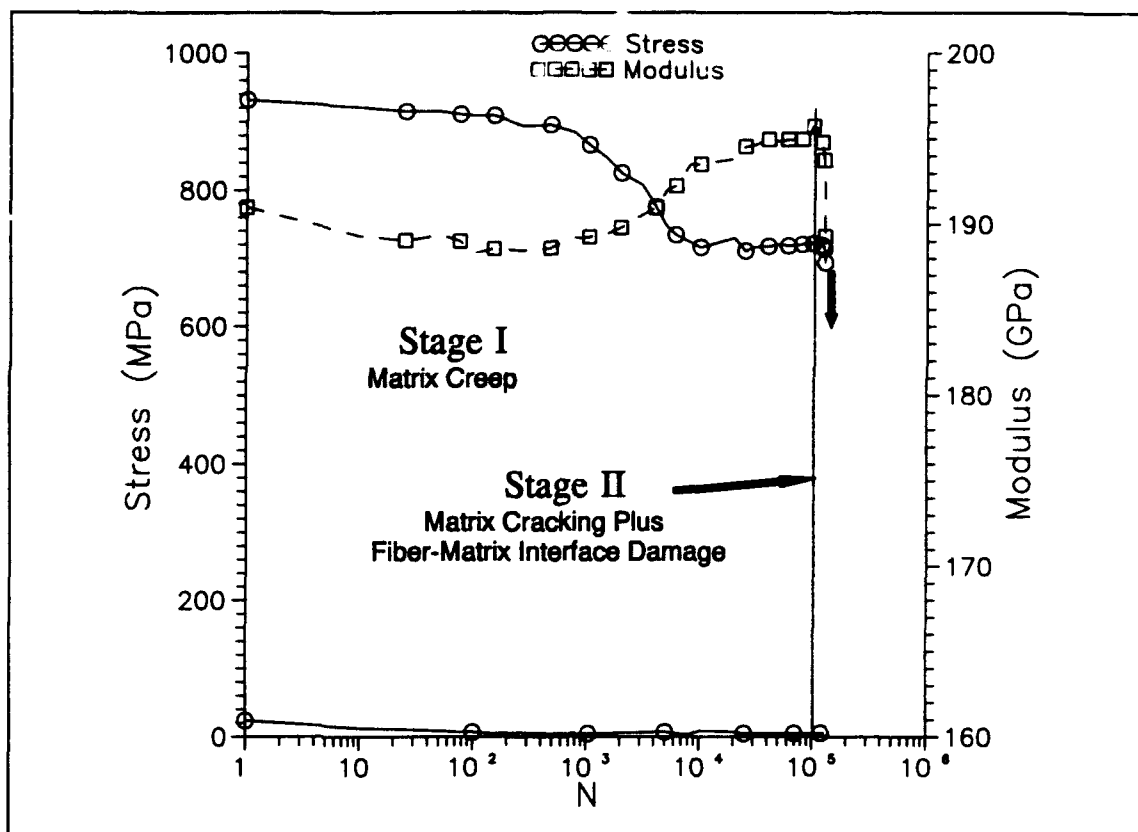
Figure A.7 0^\circ Lamina Stress and Modulus Histories, \epsilon_{\max} = .5\%
