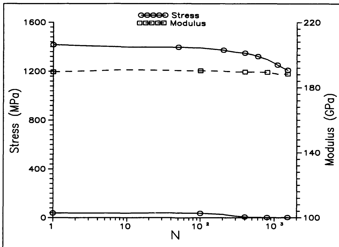
Figure 4.18 Stress and Modulus Histories for a 0^\circ Lamina, \epsilon_{\max} = .77\%
