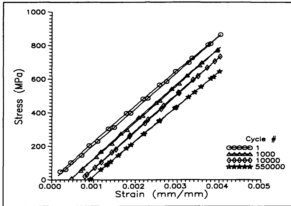
Figure A.14 0° Lamina \sigma - \epsilon History, \epsilon_{\max} = .4\%
