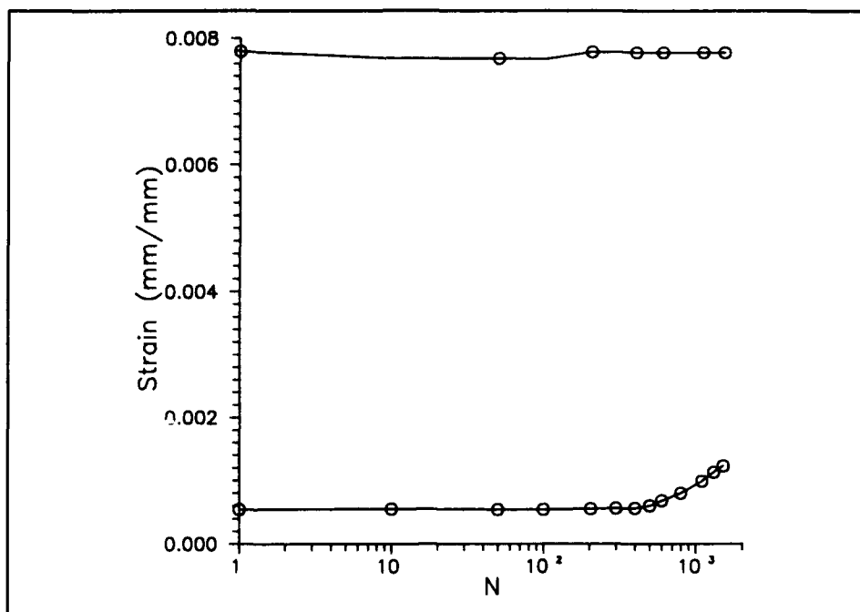
Figure A.1 0° Lamina Strain history, \epsilon_{\max} = .77\%
