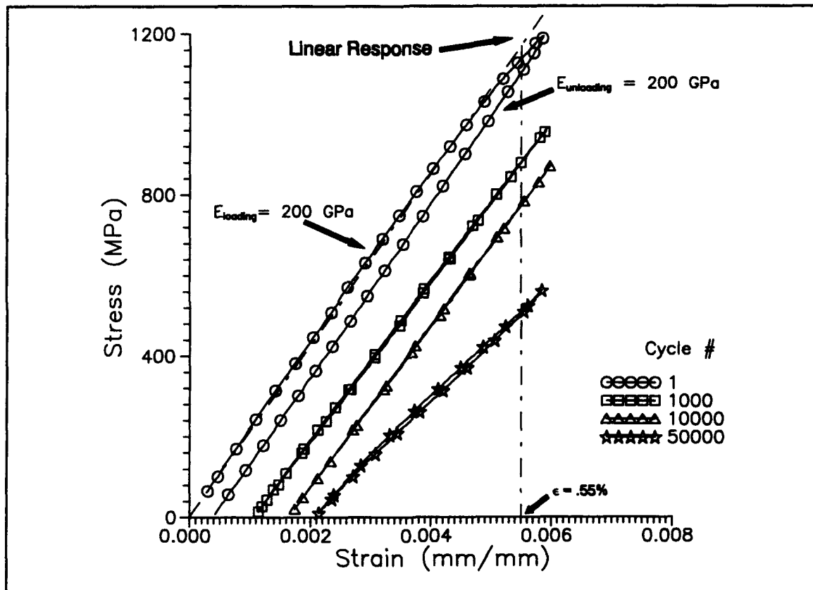
Figure 4.19 \sigma - \epsilon History for a 0^\circ Lamina, \epsilon_{\max} = .6\%
