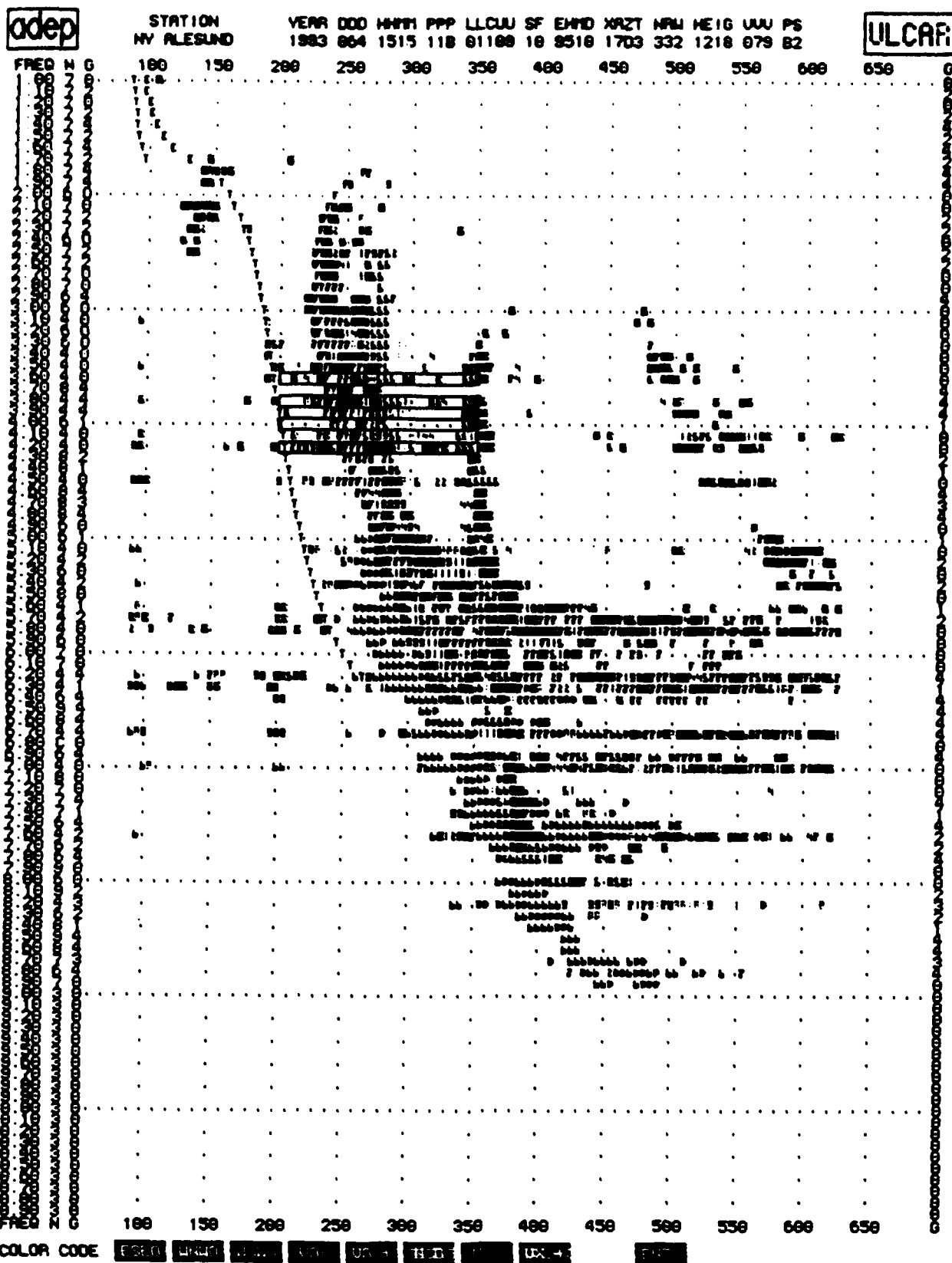
Figure 15. Digisonde ionogram recorded at 1515 UT on 5 March 1993. Darker shaded boxes display height and frequency ranges for drift measurement.
